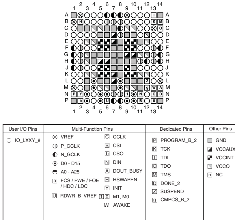
Figure 3-3: CPG196 Package—LX4, LX9, and LX16 Pinout Diagram
