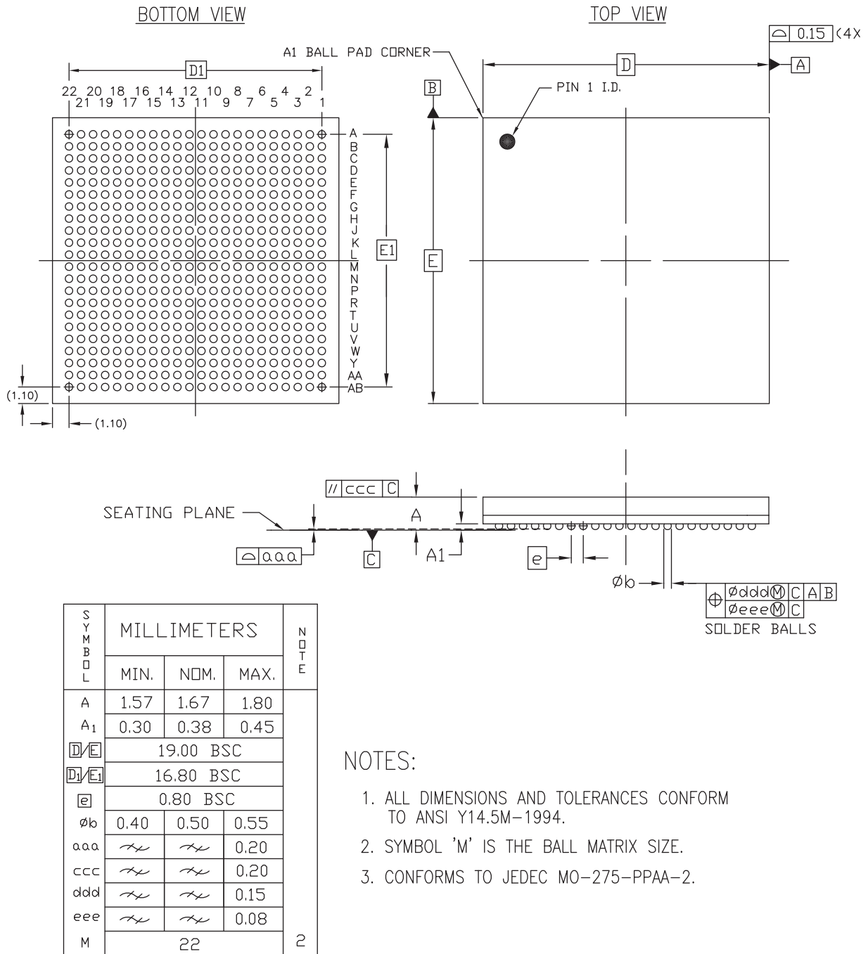
Figure 4-7: CS(G)484 Chip-Scale BGA Package
