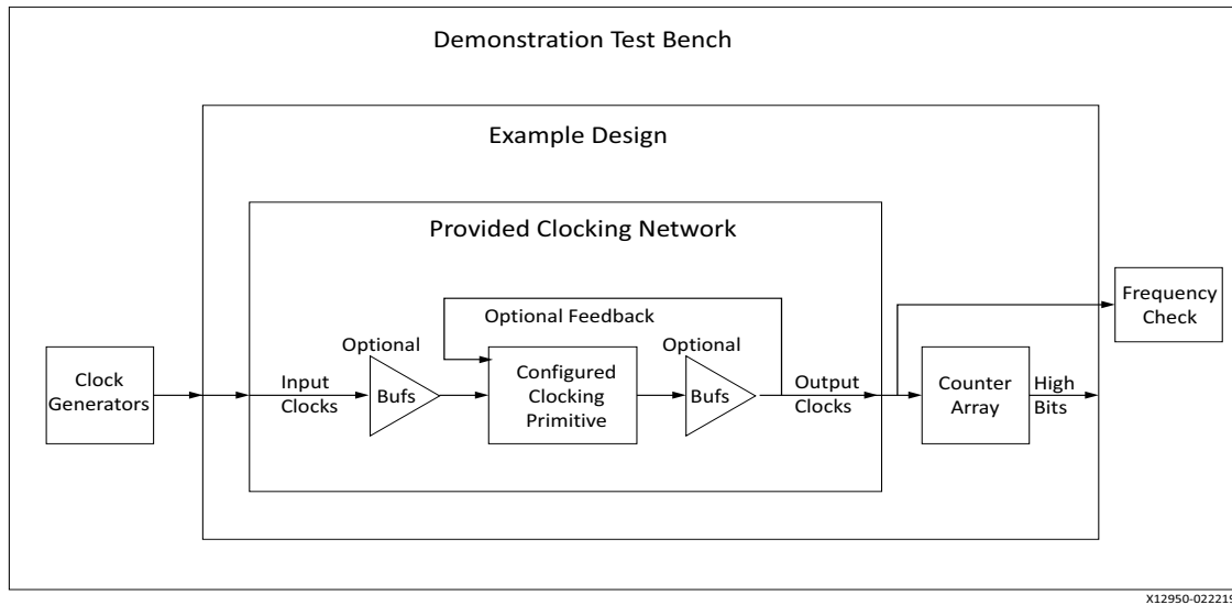
Figure 3-1: Clocking Network and Support Modules
