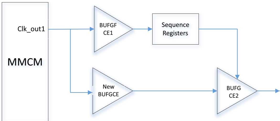
Figure C-1: Safe Clock Startup Failing Path
