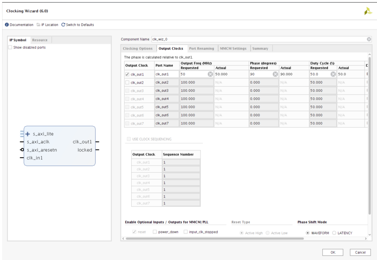
Figure 4-18: Output Clocks tab
