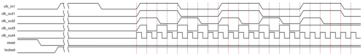
Figure 4-20: Simulation When Safe Clock Startup is True
