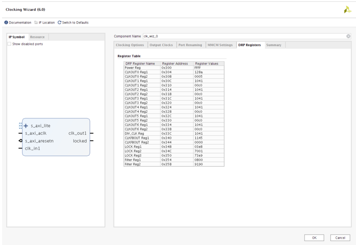
Figure 4-19: DRP Registers Tab
