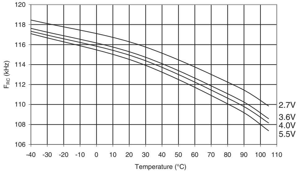
Figure 30-366. ATmega328P: Watchdog Oscillator Frequency vs. Temperature
