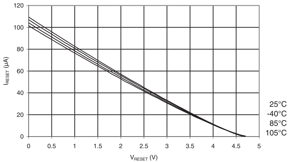
Figure 30-256. ATmega168PA: Reset Pull-up Resistor Current vs. Reset Pin Voltage ( V_{CC} = 5V )
