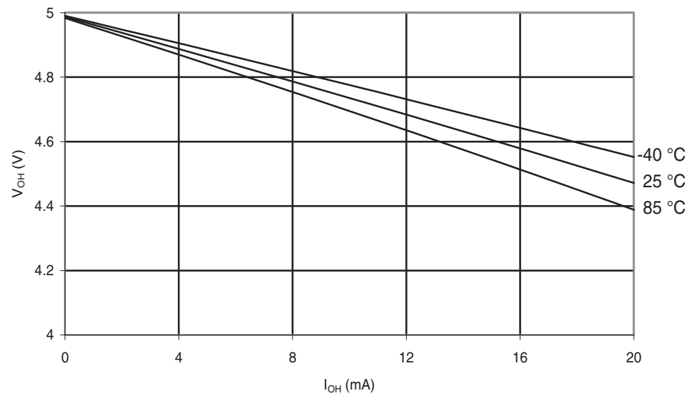
Figure 30-213. ATmega168A: I/O Pin Output Voltage vs. Source Current ( V_{CC} = 5\text{ V} )
