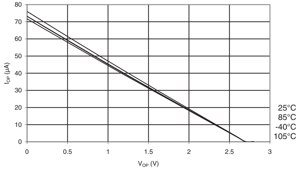
Figure 30-252. ATmega168PA: I/O Pin Pull-up Resistor Current vs. Input Voltage ( V_{CC} = 2.7V )
