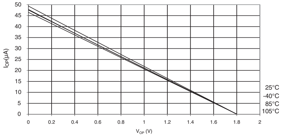
Figure 30-346. ATmega328P: I/O Pin Pull-up Resistor Current vs. Input Voltage ( V_{CC} = 1.8V )
