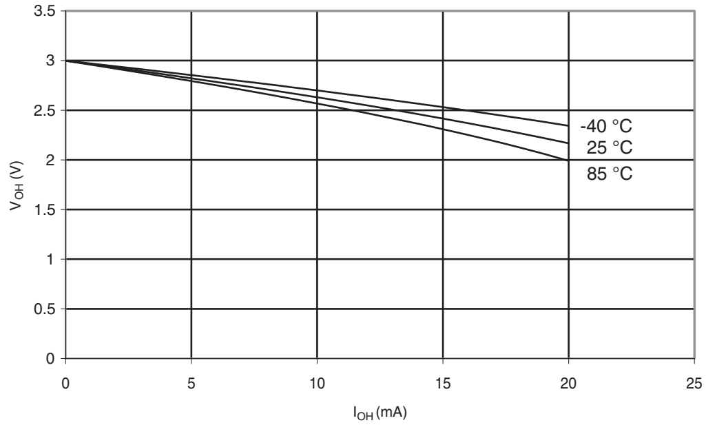
Figure 30-307. ATmega328: I/O Pin Output Voltage vs. Source Current ( V_{CC} = 3\text{ V} )
