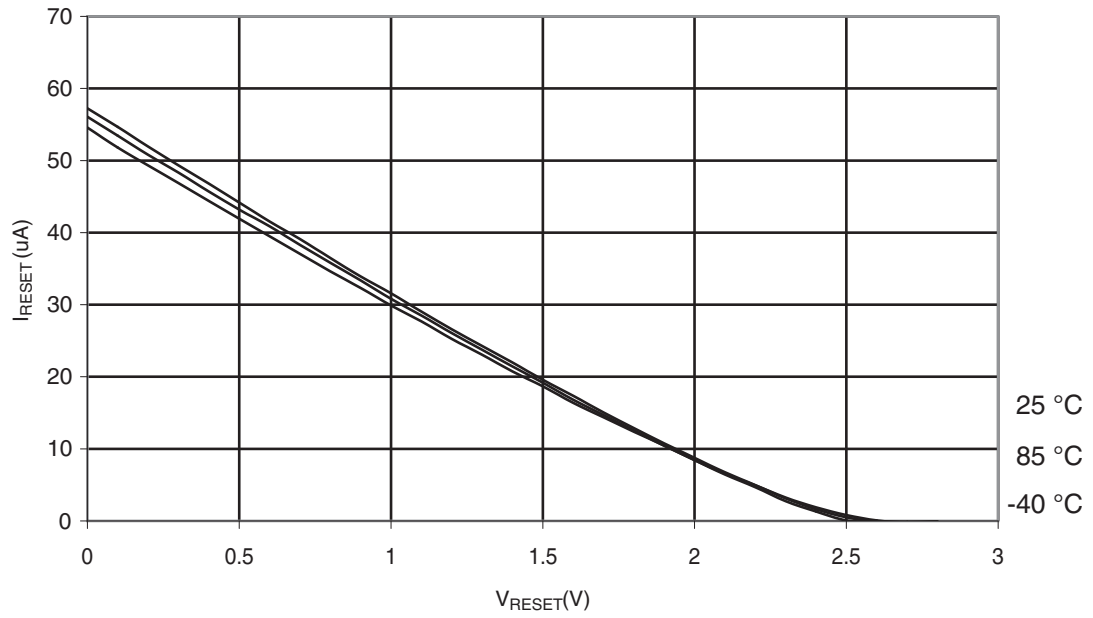
Figure 30-303. ATmega328: Reset Pull-up Resistor Current vs. Reset Pin Voltage ( V_{CC} = 2.7\text{ V} )
