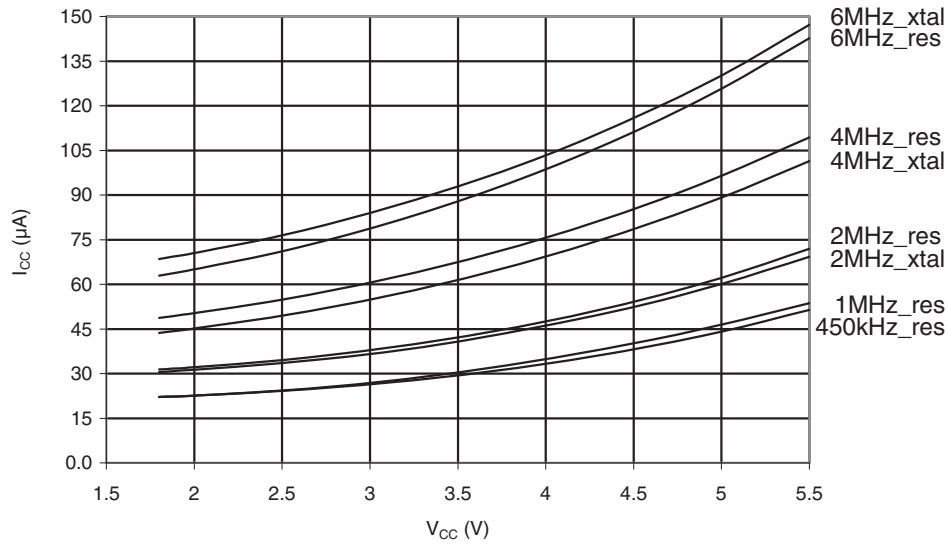
Figure 30-61. ATmega48PA: Standby Supply Current vs. V_{CC} (Watchdog Timer Disabled)
