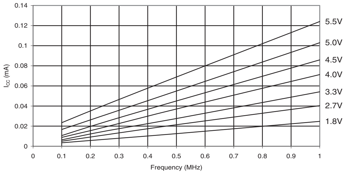
Figure 30-142. ATmega88PA: Active Supply Current vs. Low Frequency (0.1-1.0MHz)
