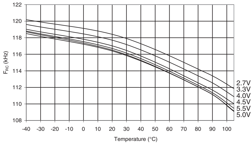
Figure 30-272. ATmega168PA: Watchdog Oscillator Frequency vs. Temperature
