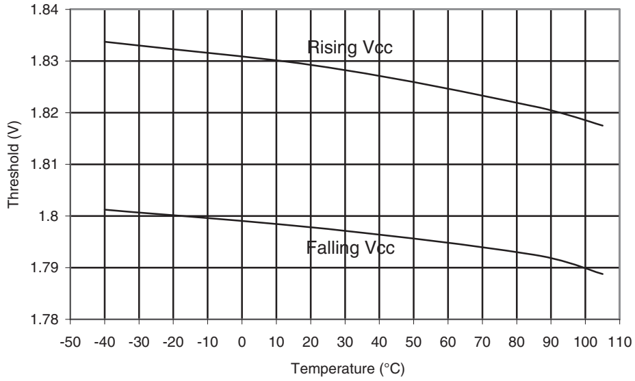
Figure 30-362. ATmega328P: BOD Thresholds vs. Temperature (BODLEVEL is 1.8V)
