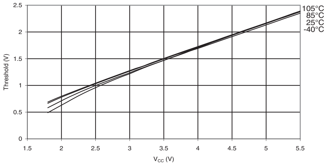
Figure 30-167. ATmega88PA: I/O Pin Input Threshold Voltage vs. V_{CC} ( V_{IL} , I/O Pin read as '0')
