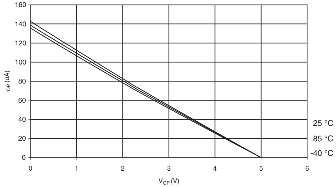
Figure 30-301. ATmega328: I/O Pin Pull-up Resistor Current vs. Input Voltage ( V_{CC} = 5\text{ V} )
