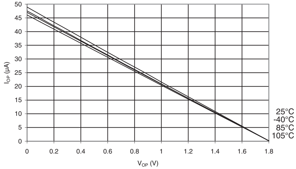
Figure 30-251. ATmega168PA: I/O Pin Pull-up Resistor Current vs. Input Voltage ( V_{CC} = 1.8V )
