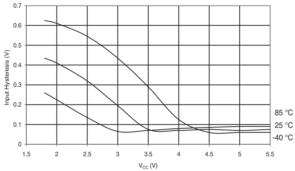
Figure 30-219. ATmega168A: Reset Pin Input Hysteresis vs. V_{CC}
