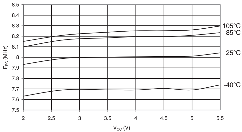
Figure 30-274. ATmega168PA: Calibrated 8MHz RC Oscillator Frequency vs. V_{CC}
