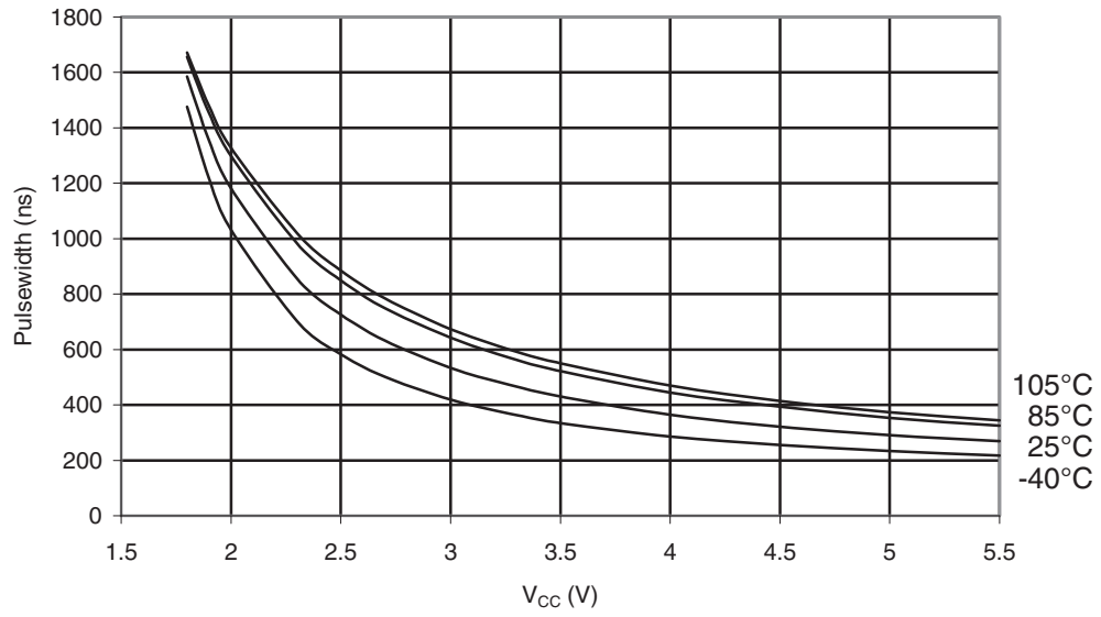
Figure 30-378. ATmega328P: Minimum Reset Pulse Width vs. V CC
