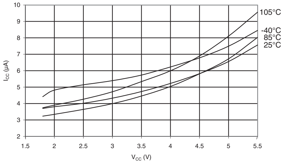
Figure 30-343. ATmega328P: Power-Down Supply Current vs. V_{CC} (Watchdog Timer Enabled)
