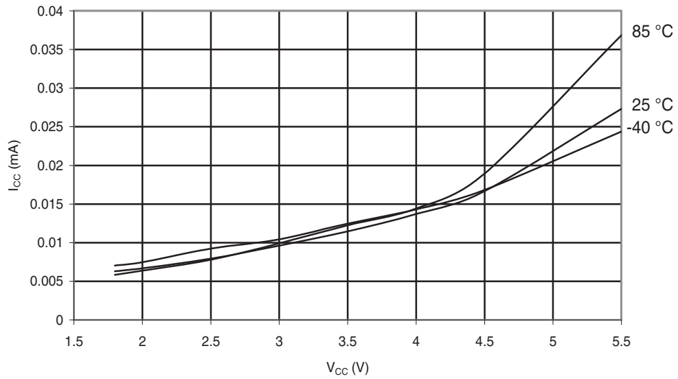
Figure 30-197. ATmega168A: Idle Supply Current vs. V_{CC} (Internal RC Oscillator, 128kHz)
