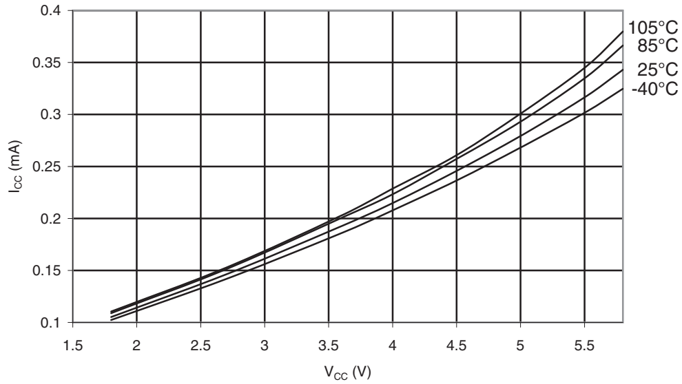
Figure 30-340. ATmega328P: Idle Supply Current vs. V_{CC} (Internal RC Oscillator, 1MHz)
