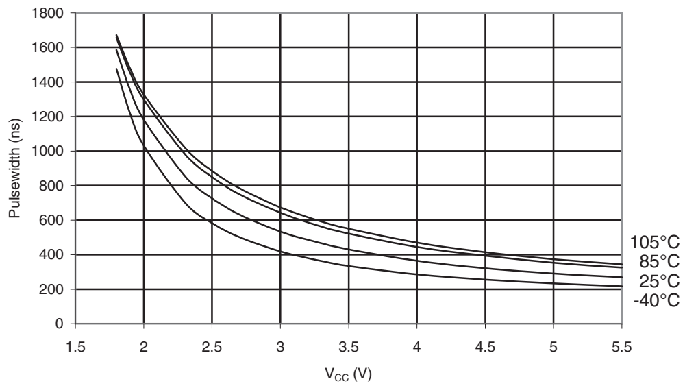
Figure 30-284. ATmega168PA: Minimum Reset Pulse Width vs. V_{CC}
