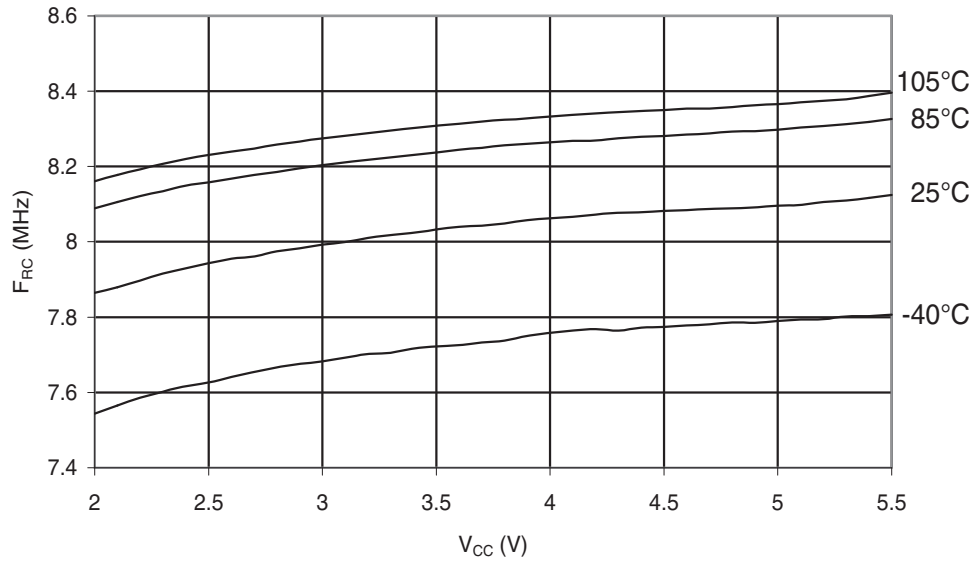
Figure 30-368. ATmega328P: Calibrated 8 MHz RC Oscillator Frequency vs. V_{CC}
