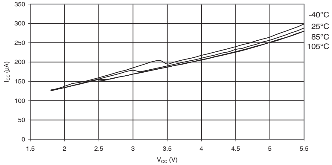
Figure 30-183. ATmega88PA: Analog Comparator Current vs. V_{CC}
