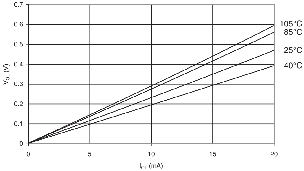
Figure 30-353. ATmega328P: I/O Pin Output Voltage vs. Sink Current ( V_{CC} = 5V )
