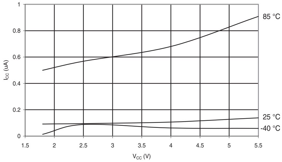
Figure 30-201. ATmega168A: Power-Down Supply Current vs. V_{CC} (Watchdog Timer Enabled)
