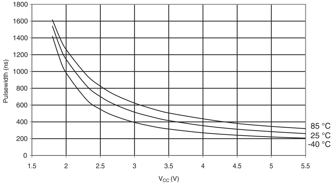
Figure 30-331. ATmega328: Minimum Reset Pulse width vs. V_{CC}
