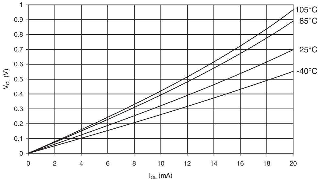
Figure 30-69. ATmega48PA: I/O Pin Output Voltage vs. Sink Current ( V_{CC} = 5V )
