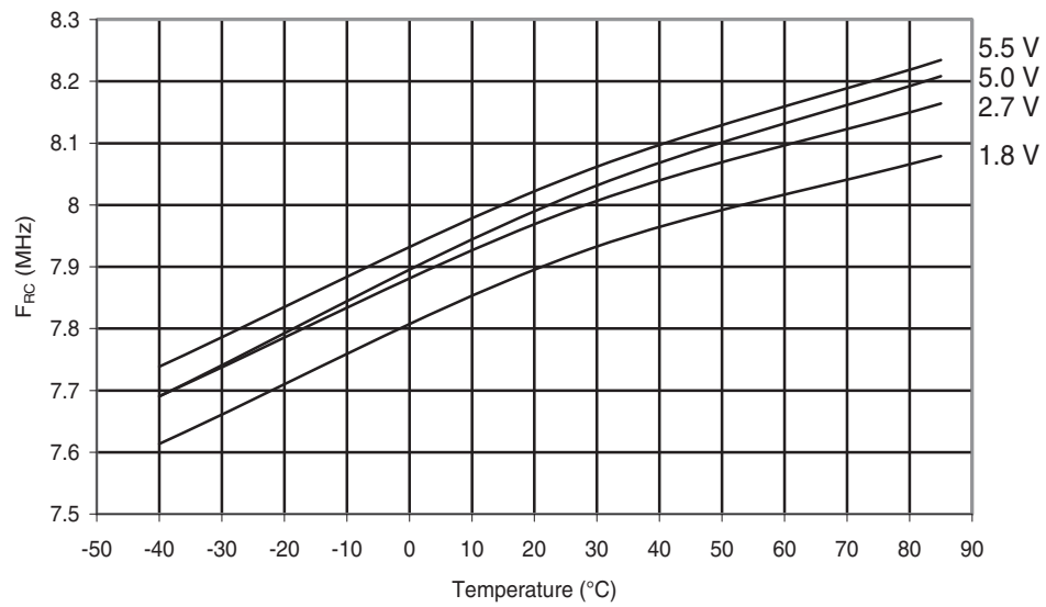
Figure 30-227. ATmega168A: Calibrated 8MHz RC Oscillator Frequency vs. Temperature
