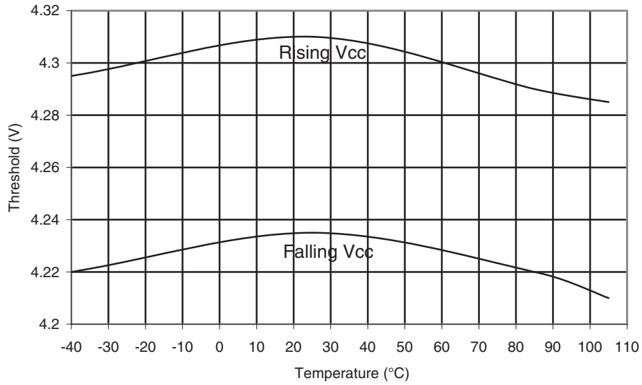
Figure 30-269. ATmega168PA: BOD Thresholds vs. Temperature (BODLEVEL is 4.3V)
