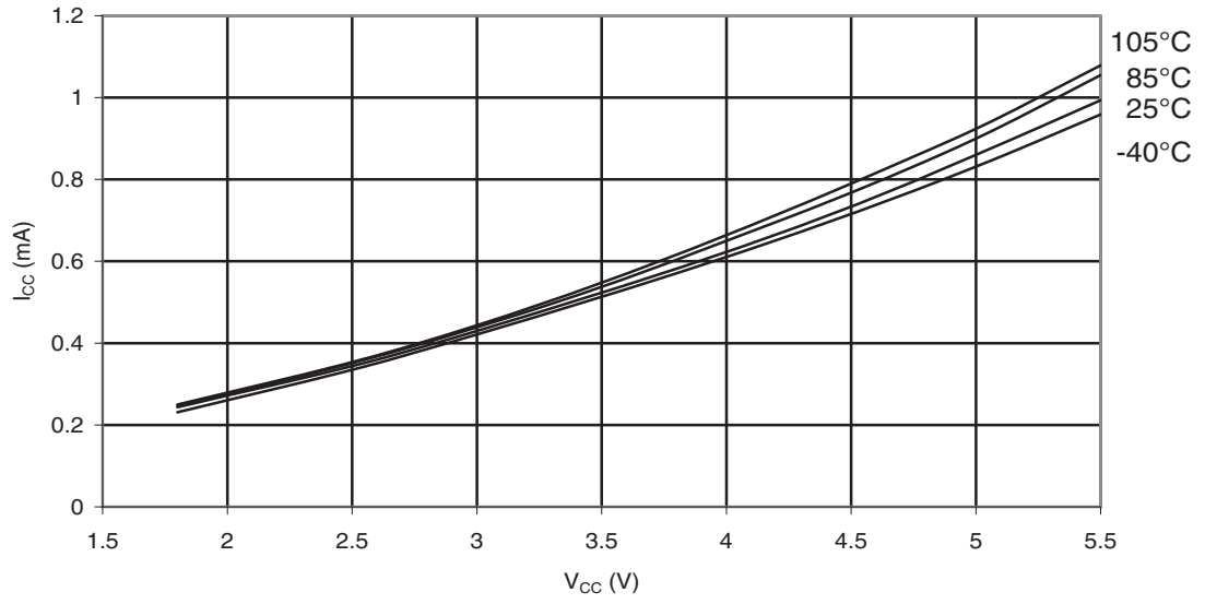
Figure 30-151. ATmega88PA: Idle Supply Current vs. V_{CC} (Internal RC Oscillator, 8MHz)
