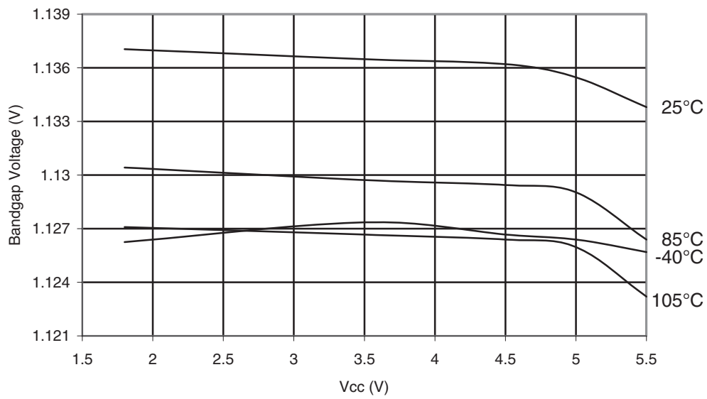
Figure 30-365. ATmega328P: Calibrated Bandgap Voltage vs. Vcc
