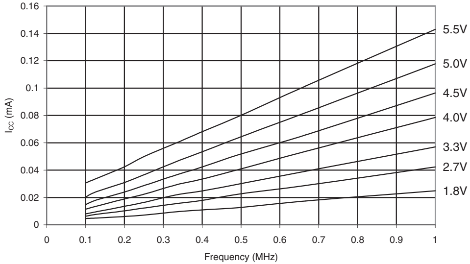
Figure 30-48. ATmega48PA: Active Supply Current vs. Low Frequency (0.1-1.0MHz)
