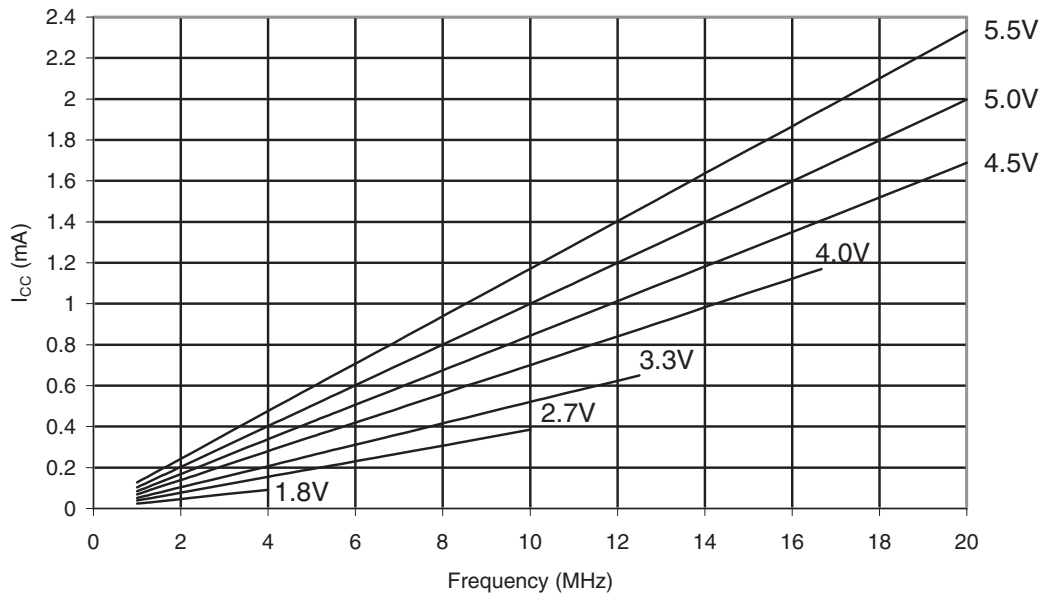
Figure 30-93. ATmega48PA: Reset Supply Current vs. Frequency (1MHz- 20MHz)
