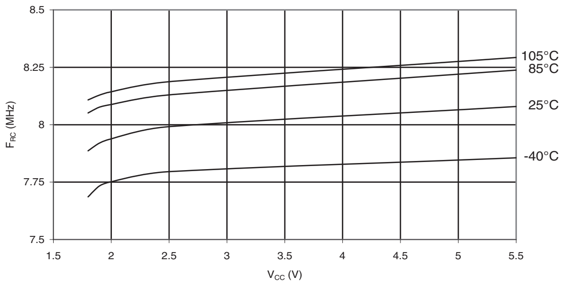
Figure 30-179. ATmega88PA: Calibrated 8MHz RC Oscillator Frequency vs. V_{CC}
