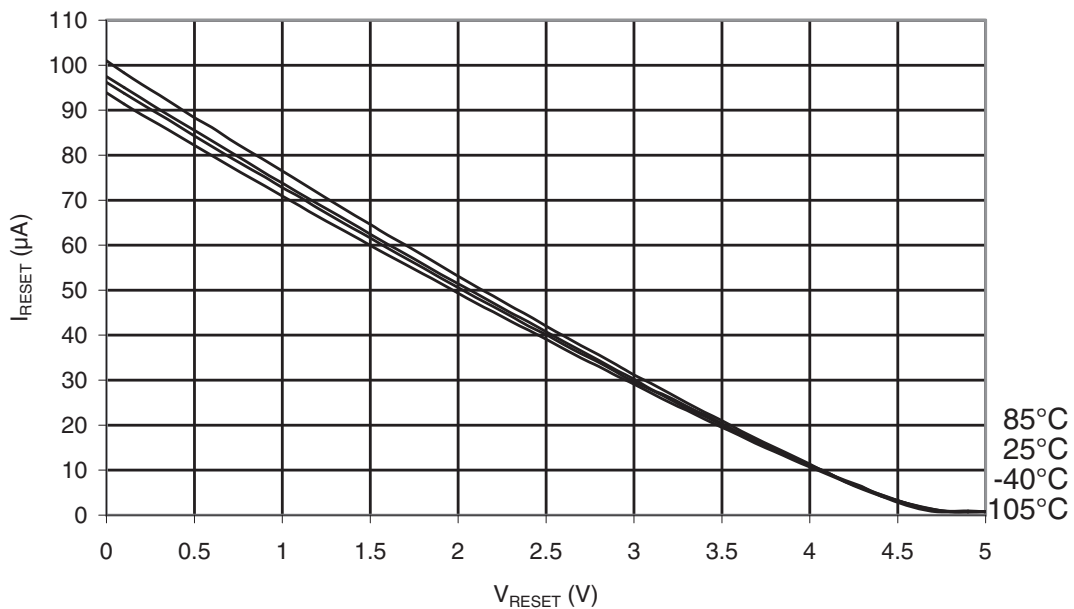
Figure 30-67. ATmega48PA: Reset Pull-up Resistor Current vs. Reset Pin Voltage ( V_{CC} = 5V )
