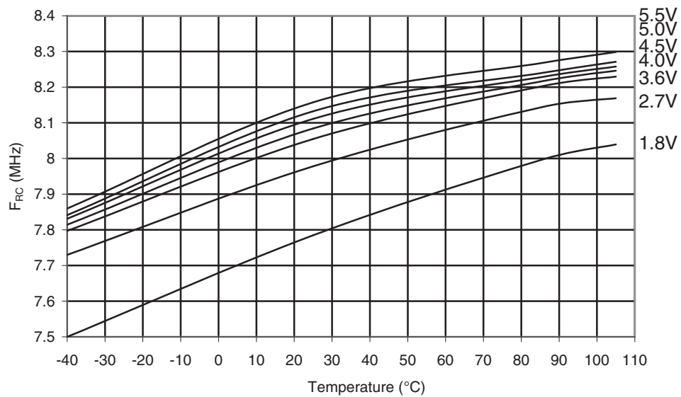
Figure 30-369. ATmega328P: Calibrated 8MHz RC Oscillator Frequency vs. Temperature
