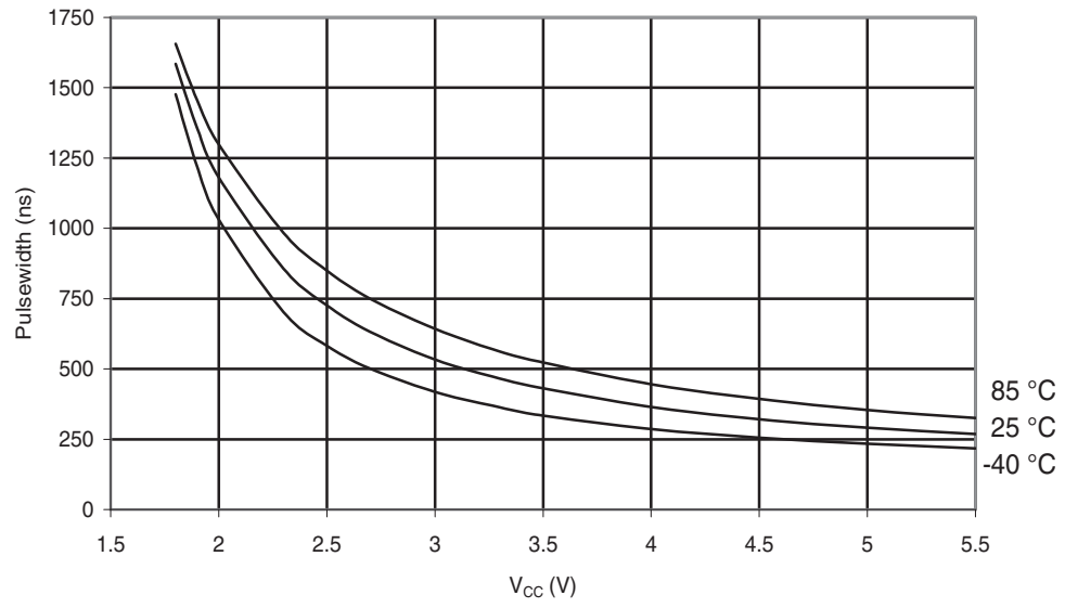
Figure 30-236. ATmega168A: Minimum Reset Pulse width vs. V_{CC}
