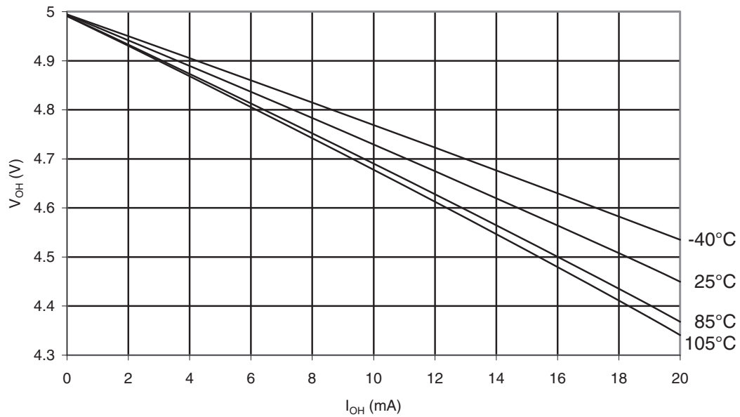
Figure 30-71. ATmega48PA: I/O Pin Output Voltage vs. Source Current ( V_{CC} = 5V )
