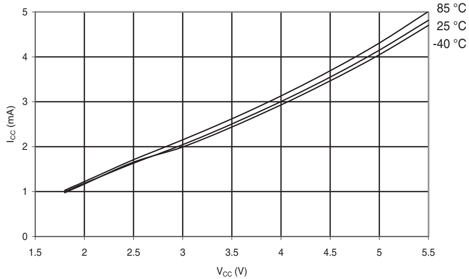
Figure 30-194. ATmega168A: Active Supply Current vs. V_{CC} (Internal RC Oscillator, 8MHz)
