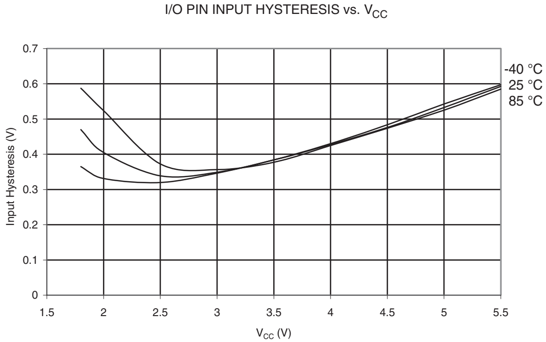
Figure 30-311. ATmega328: I/O Pin Input Hysteresis vs. V_{CC}
