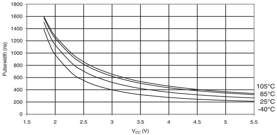
Figure 30-189. ATmega88PA: Minimum Reset Pulse width vs. V_{CC}
