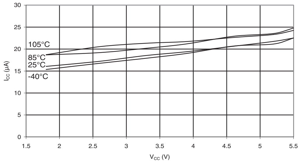
Figure 30-185. ATmega88PA: Brownout Detector Current vs. V_{CC}
