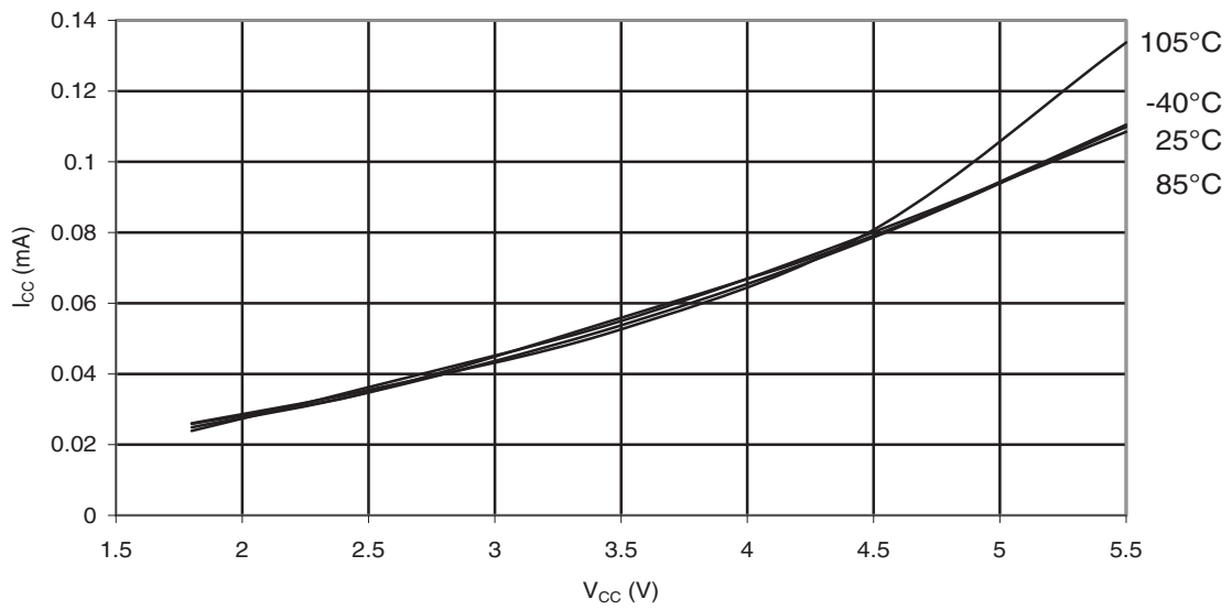
Figure 30-144. ATmega88PA: Active Supply Current vs. V_{CC} (Internal RC Oscillator, 128kHz)
