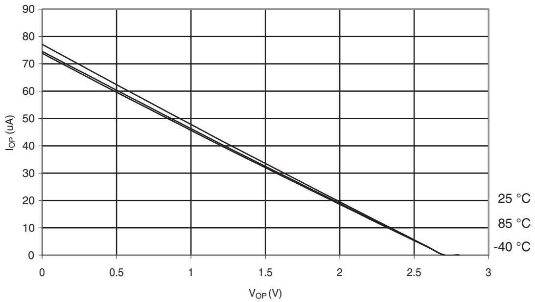
Figure 30-300. ATmega328: I/O Pin Pull-up Resistor Current vs. Input Voltage ( V_{CC} = 2.7\text{ V} )
