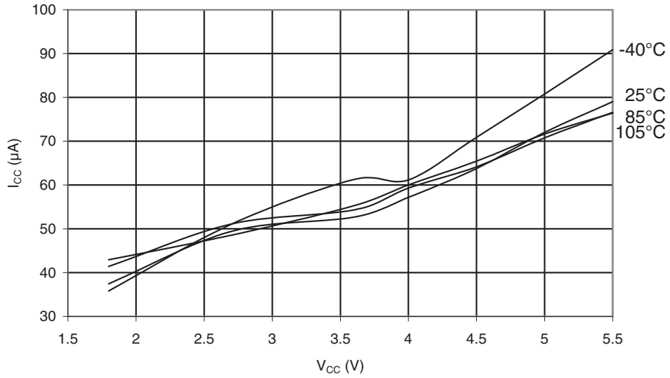
Figure 30-372. ATmega328P: Analog Comparator Current vs. V_{CC}
