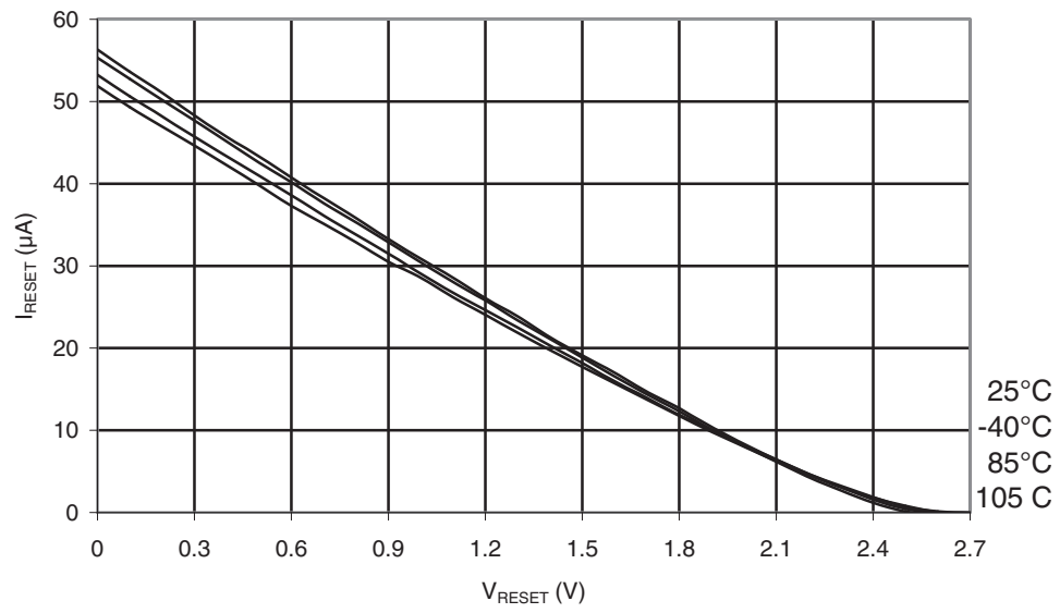
Figure 30-256. ATmega168PA: Reset Pull-up Resistor Current vs. Reset Pin Voltage ( V_{CC} = 5V )
