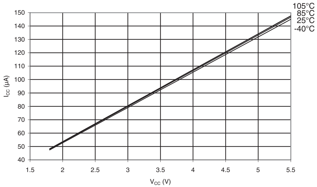
Figure 30-89. ATmega48PA: AREF External Reference Current vs. V_{CC}
