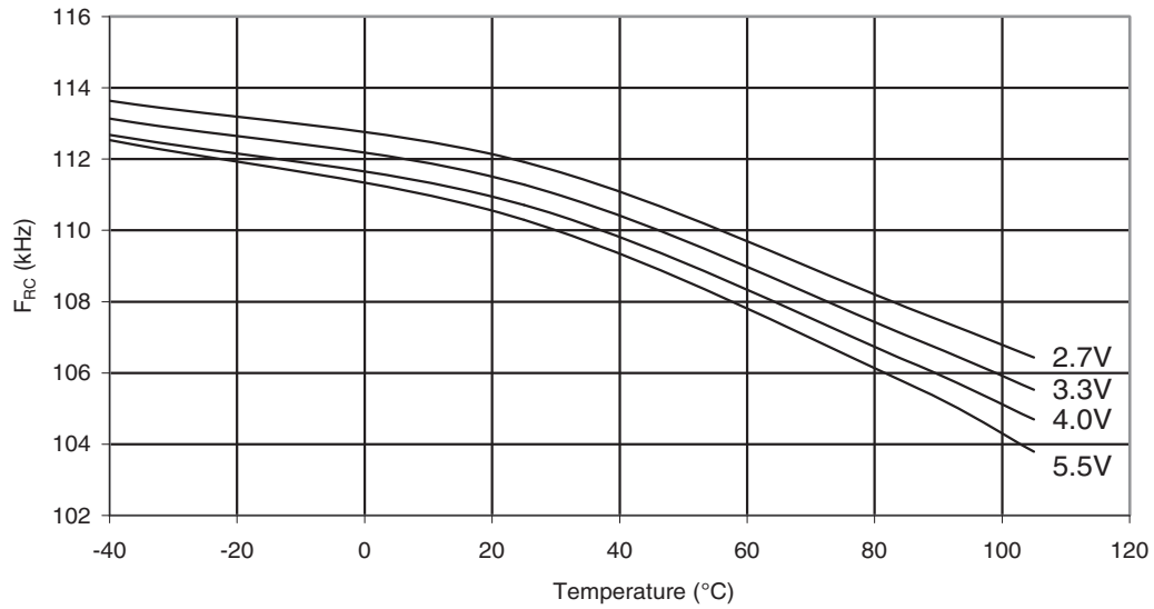
Figure 30-177. ATmega88PA: Watchdog Oscillator Frequency vs. Temperature
