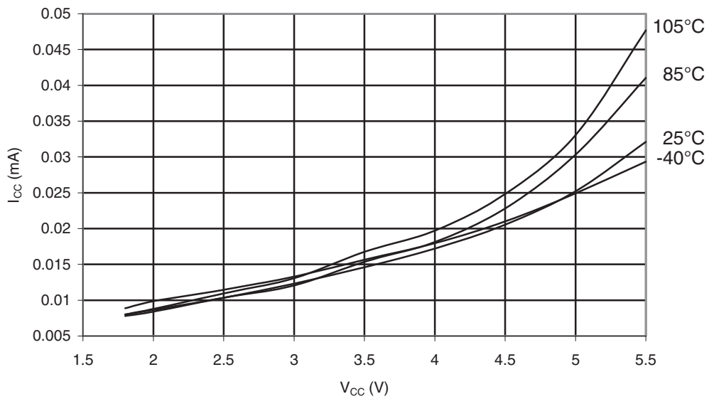
Figure 30-339. ATmega328P: Idle Supply Current vs. V_{CC} (Internal RC Oscillator, 128kHz)
