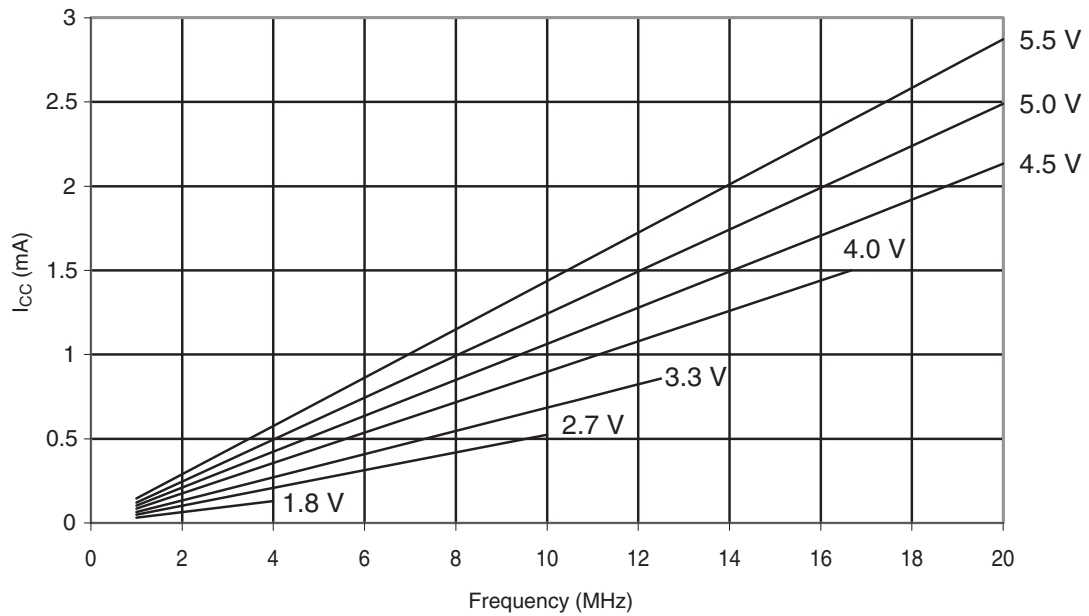
Figure 30-330. ATmega328: Reset Supply Current vs. Frequency (1 - 20MHz)
