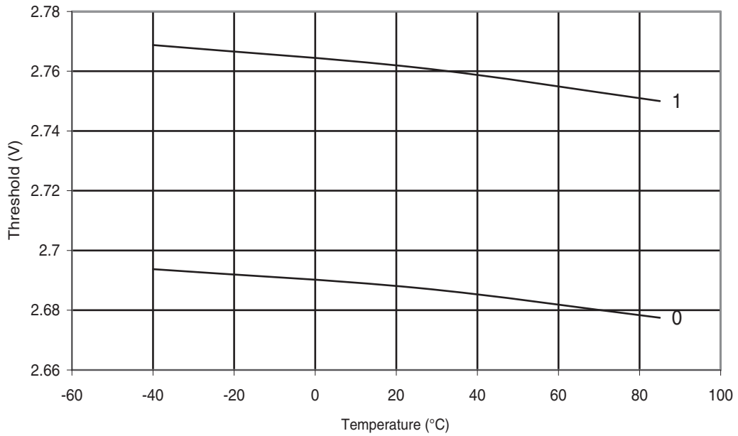
Figure 30-316. ATmega328: BOD Thresholds vs. Temperature (BODLEVEL is 2.7 V)
