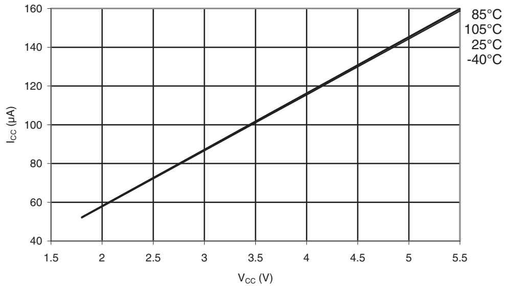
Figure 30-371. ATmega328P: ADC Current vs. V_{CC} (AREF = AV_{CC} )
