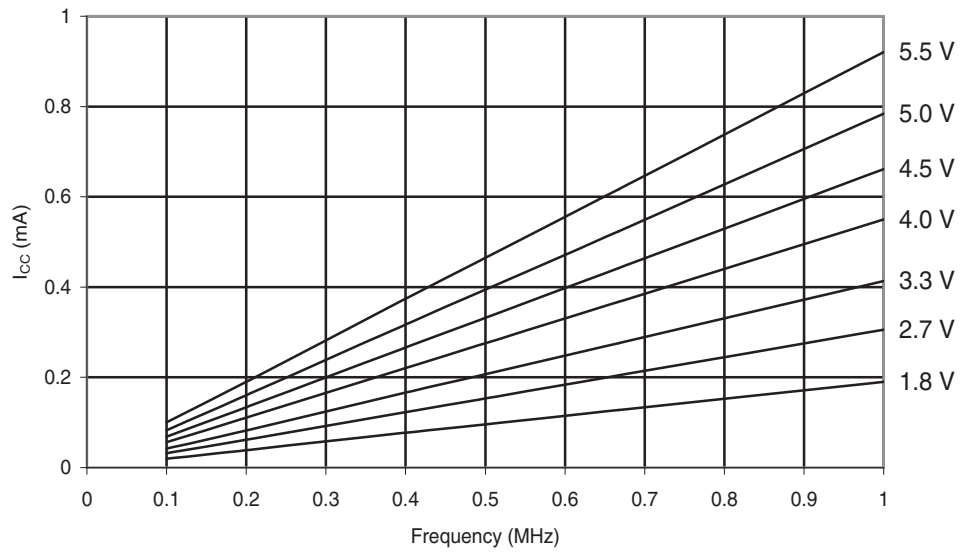
Figure 30-190. ATmega168A: Active Supply Current vs. Low Frequency (0.1-1.0MHz)
