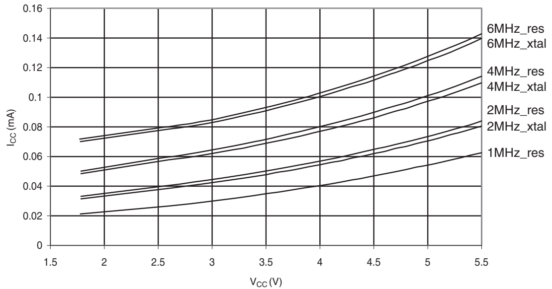
Figure 30-345. ATmega328P: Standby Supply Current vs. V_{CC} (Watchdog Timer Disabled)
