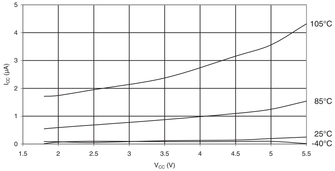
Figure 30-153. ATmega88PA: Power-Down Supply Current vs. V_{CC} (Watchdog Timer Enabled)
