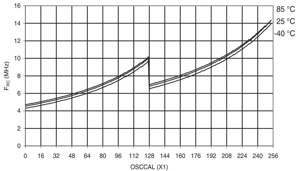
Figure 30-228. ATmega168A: Calibrated 8MHz RC Oscillator Frequency vs. OSCCAL Value
