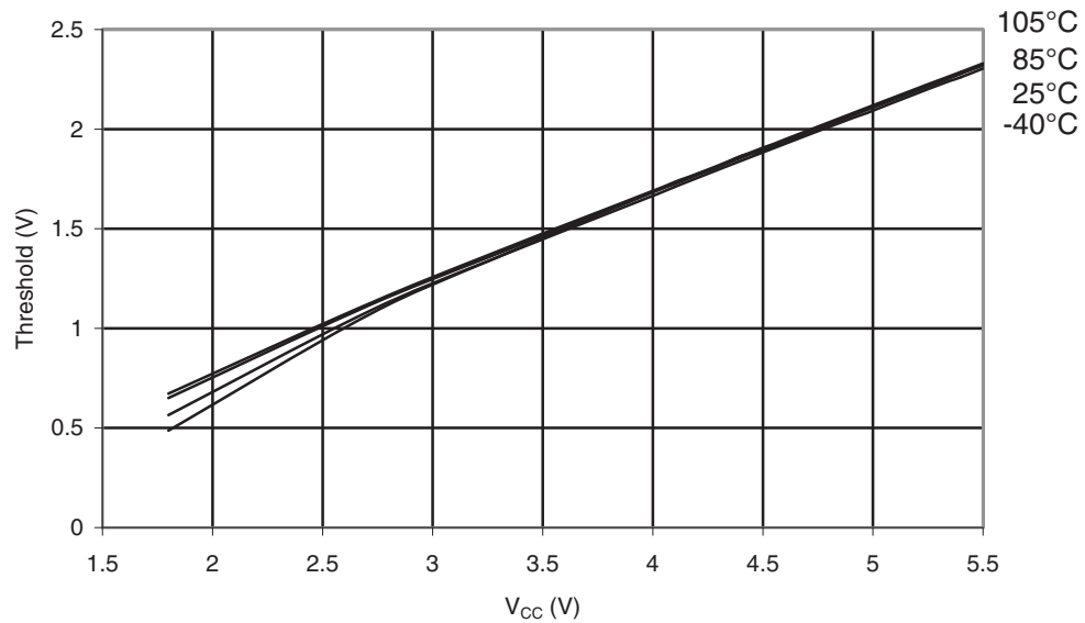
Figure 30-262. ATmega168PA I/O Pin Input Threshold Voltage vs. V_{CC} ( V_{IL} , I/O Pin read as '0')
