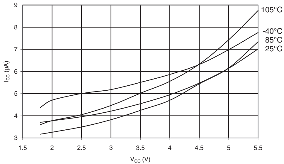
Figure 30-248. ATmega168PA: Power-Down Supply Current vs. V_{CC} (Watchdog Timer Enabled)
