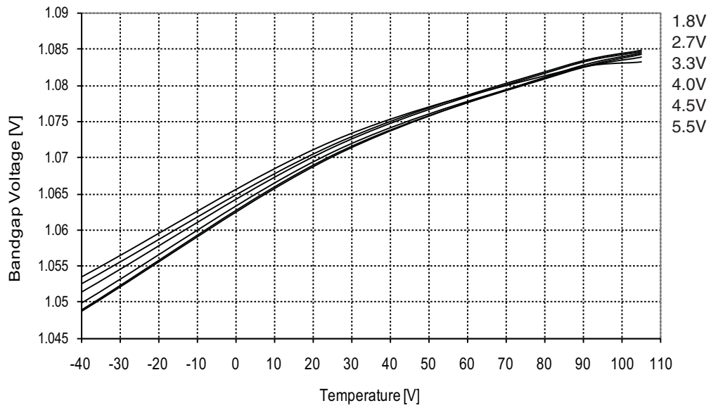
Figure 30-175. ATmega88PA: Calibrated Bandgap Voltage vs. Temperature
