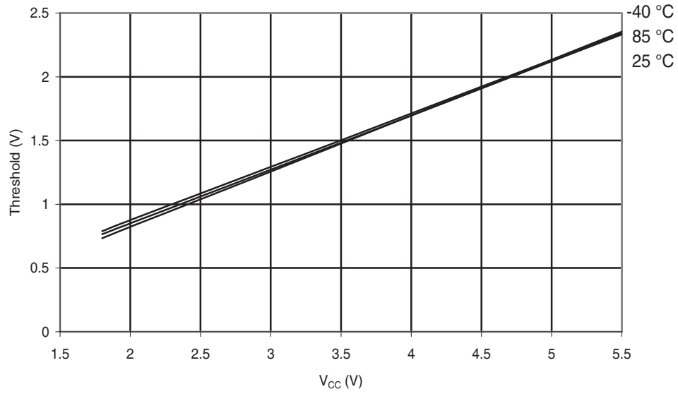
Figure 30-218. ATmega168A: Reset Input Threshold Voltage vs. V_{CC} ( V_{IL} , I/O Pin read as '0')
