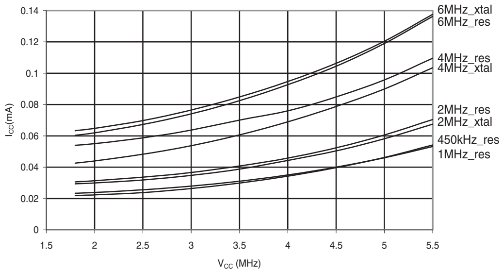
Figure 30-250. ATmega168PA: Standby Supply Current vs. V_{CC} (Watchdog Timer Disabled)
