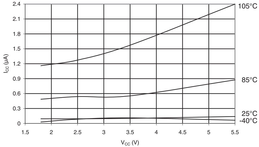
Figure 30-247. ATmega168PA: Power-Down Supply Current vs. V_{CC} (Watchdog Timer Disabled)
