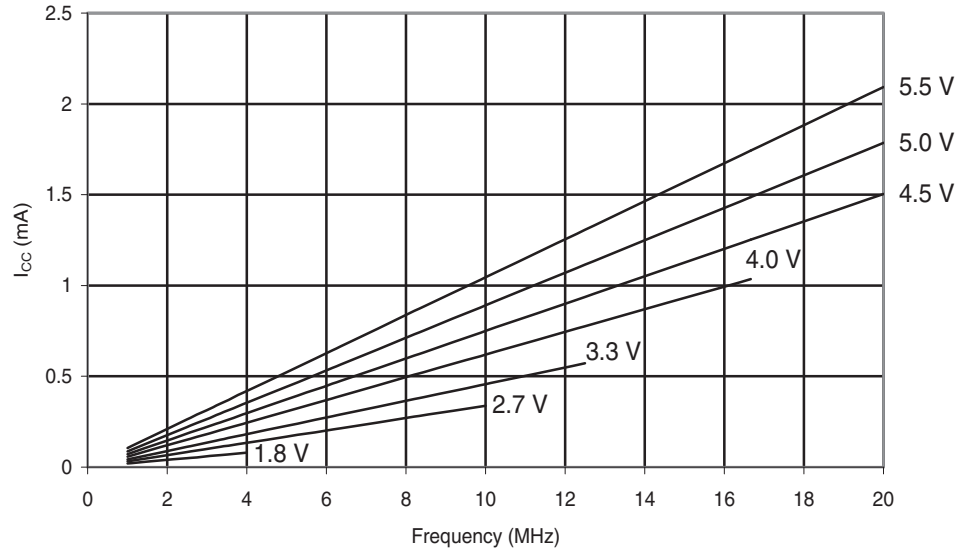
Figure 30-235. ATmega168A: Reset Supply Current vs. Frequency (1 - 20MHz)
