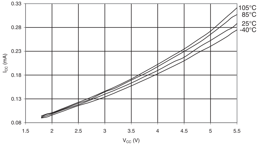
Figure 30-57. ATmega48PA: Idle Supply Current vs. V_{CC} (Internal RC Oscillator, 8MHz)
