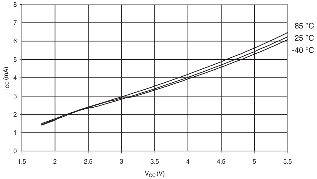
Figure 30-289. ATmega328: Active Supply Current vs. V_{CC} (Internal RC Oscillator, 8MHz)
