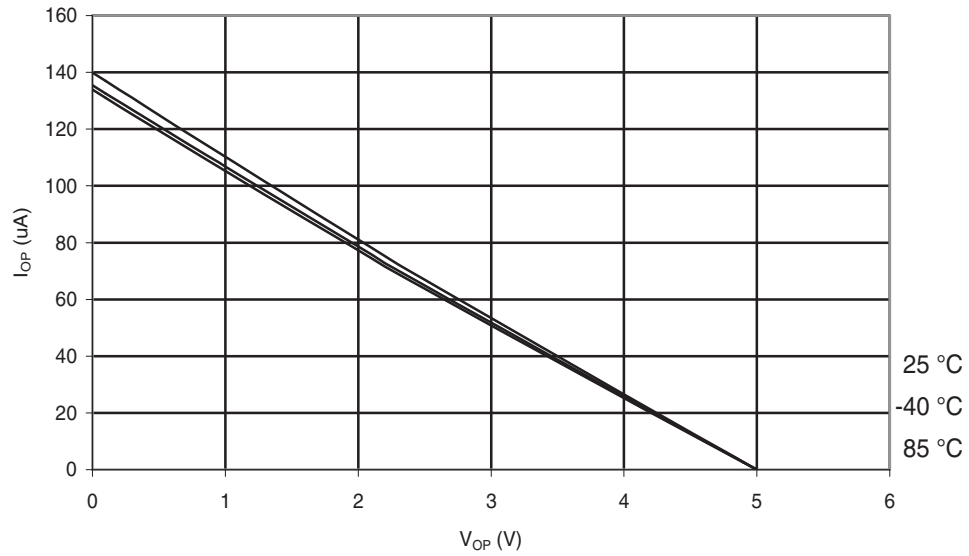
Figure 30-206. ATmega168A: I/O Pin Pull-up Resistor Current vs. Input Voltage ( V_{CC} = 5\text{ V} )
