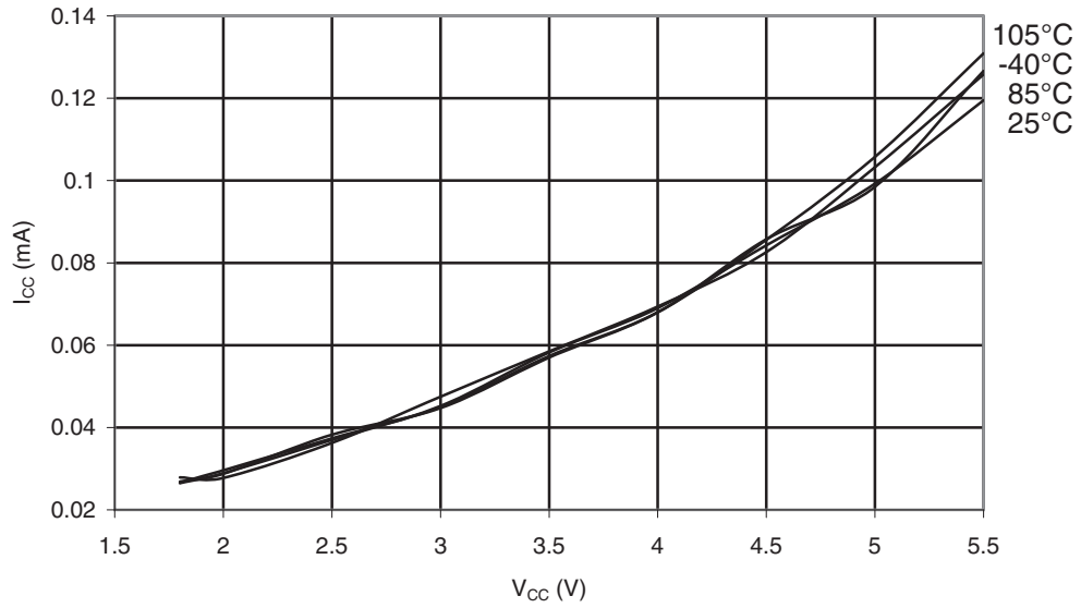
Figure 30-240. ATmega168PA: Active Supply Current vs. V_{CC} (Internal RC Oscillator, 1MHz)
