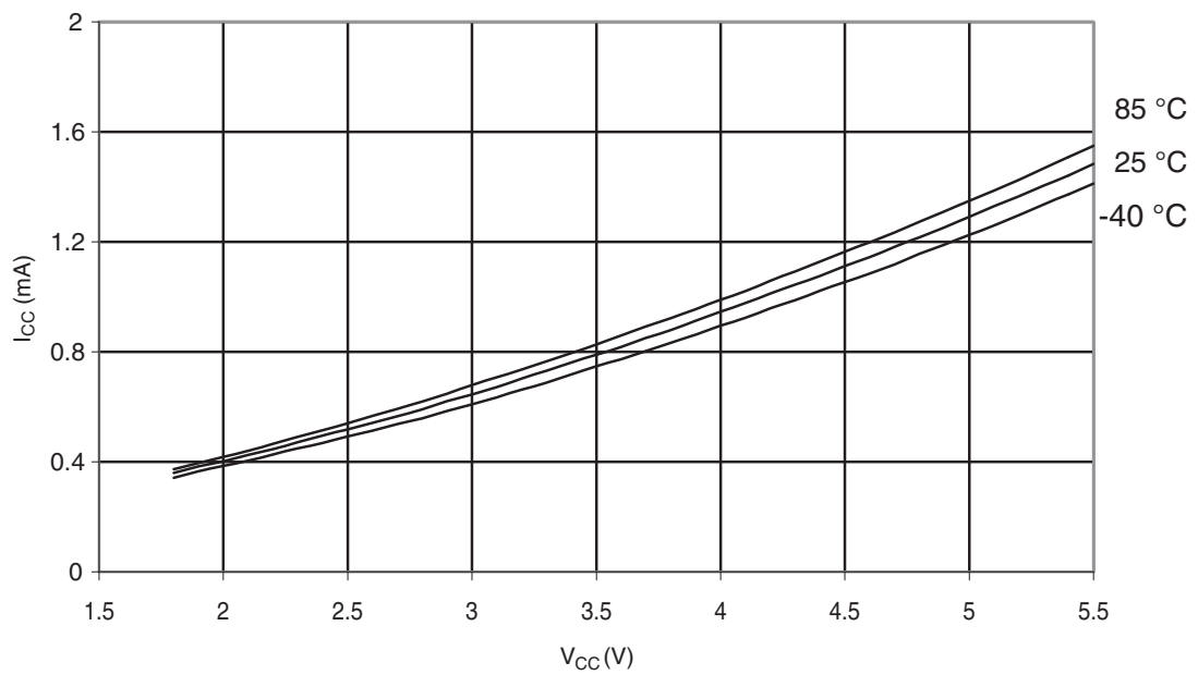
Figure 30-294. ATmega328: Idle Supply Current vs. V_{CC} (Internal RC Oscillator, 8MHz)
