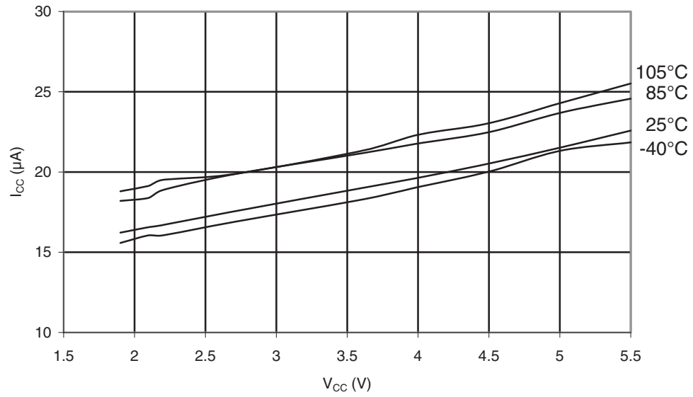
Figure 30-374. ATmega328P: Brownout Detector Current vs. V_{CC}
