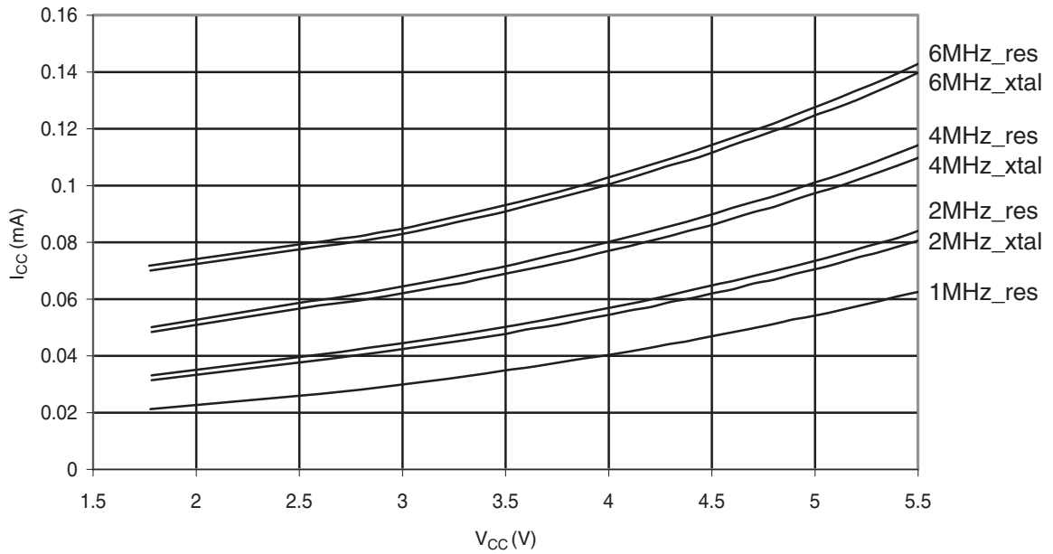
Figure 30-298. ATmega328: Standby Supply Current vs. V_{CC} (Watchdog Timer Disabled)
