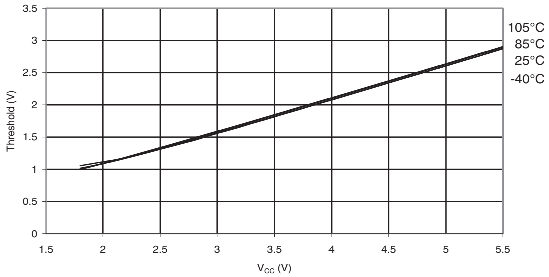
Figure 30-166. ATmega88PA: I/O Pin Input Threshold Voltage vs. V_{CC} ( V_{IH} , I/O Pin read as '1')
