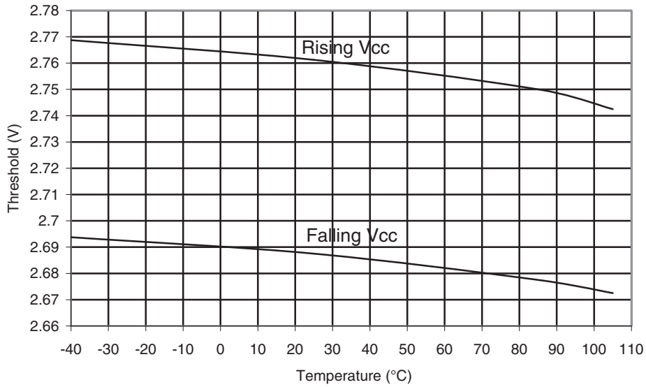
Figure 30-363. ATmega328P BOD Thresholds vs. Temperature (BODLEVEL is 2.7V)
