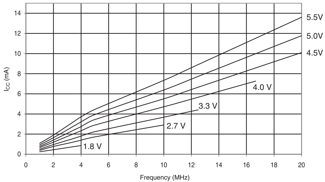
Figure 30-286. ATmega328: Active Supply Current vs. Frequency (1-20MHz)
