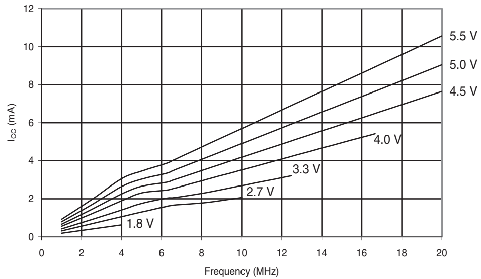
Figure 30-191. ATmega168A: Active Supply Current vs. Frequency (1-20MHz)
