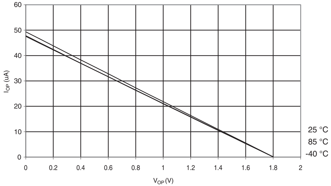
Figure 30-299. ATmega328: I/O Pin Pull-up Resistor Current vs. Input Voltage ( V_{CC} = 1.8\text{ V} )
