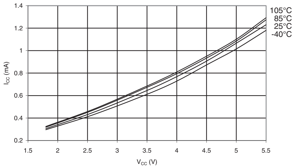
Figure 30-335. ATmega328P: Active Supply Current vs. V_{CC} (Internal RC Oscillator, 1MHz)
