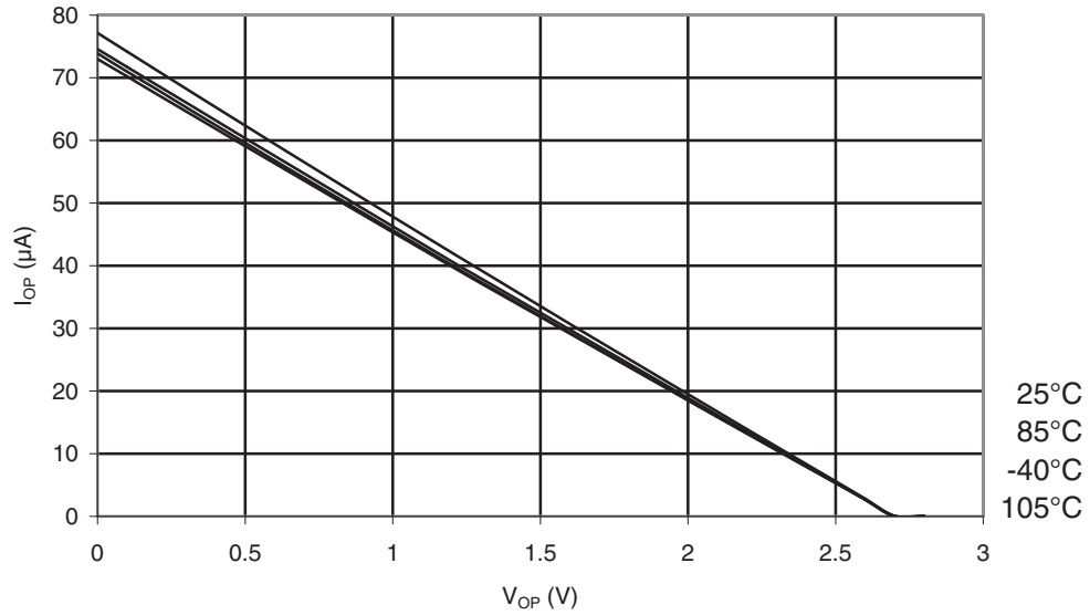
Figure 30-347. ATmega328P: I/O Pin Pull-up Resistor Current vs. Input Voltage ( V_{CC} = 2.7V )
