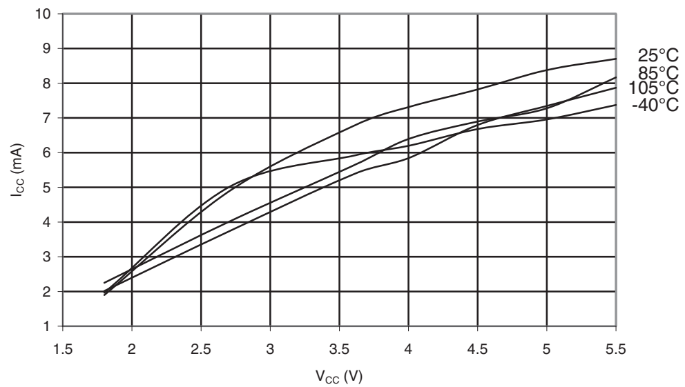
Figure 30-375. ATmega328P: Programming Current vs. V_{CC}
