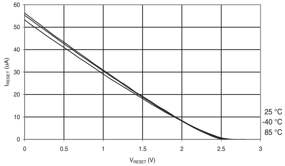
Figure 30-208. ATmega168A: Reset Pull-up Resistor Current vs. Reset Pin Voltage ( V_{CC} = 2.7\text{ V} )
