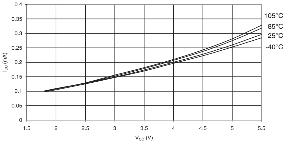
Figure 30-150. ATmega88PA: Idle Supply Current vs. V_{CC} (Internal RC Oscillator, 1MHz)
