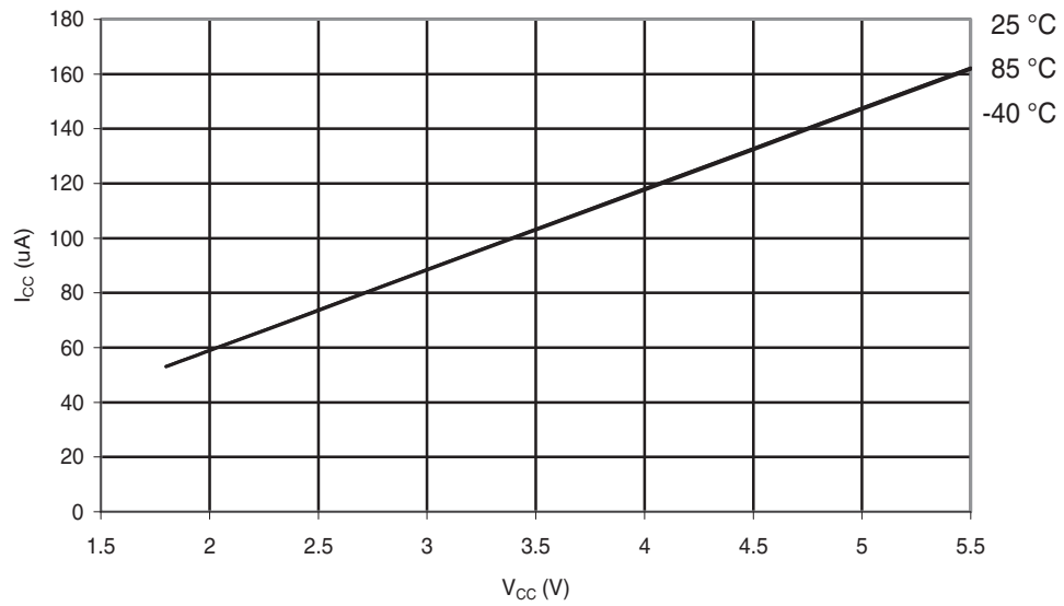
Figure 30-231. ATmega168A: AREF External Reference Current vs. V_{CC}
