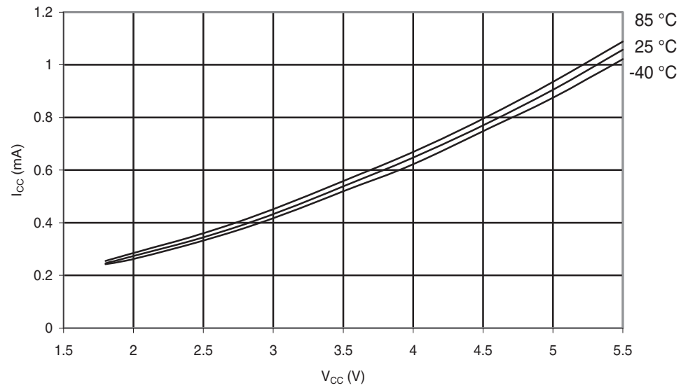
Figure 30-193. ATmega168A: Active Supply Current vs. V_{CC} (Internal RC Oscillator, 1MHz)
