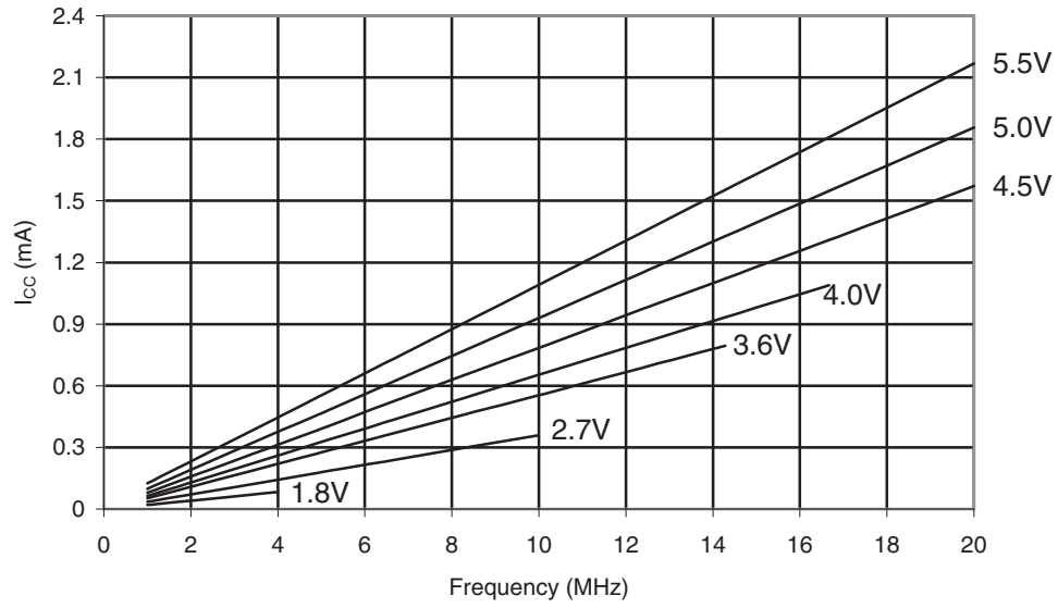
Figure 30-283. ATmega168PA: Reset Supply Current vs. Frequency (1MHz - 20MHz)
