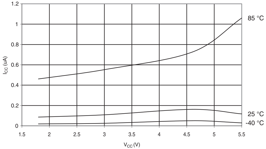
Figure 30-295. ATmega328: Power-Down Supply Current vs. V_{CC} (Watchdog Timer Disabled)
