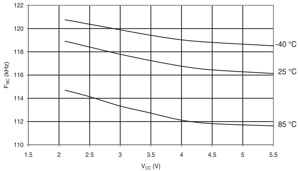
Figure 30-225. ATmega168A: Watchdog Oscillator Frequency vs. V_{CC}
