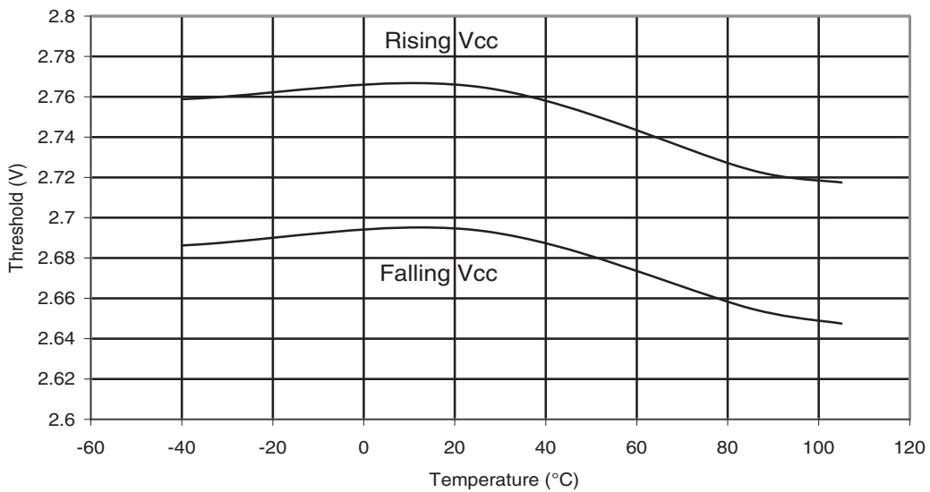
Figure 30-173. ATmega88PA: BOD Thresholds vs. Temperature (BODLEVEL is 2.7V)
