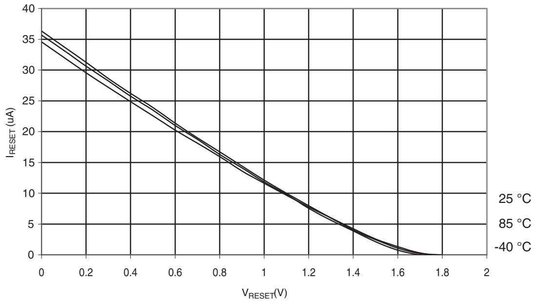
Figure 30-302. ATmega328: Reset Pull-up Resistor Current vs. Reset Pin Voltage ( V_{CC} = 1.8\text{ V} )
