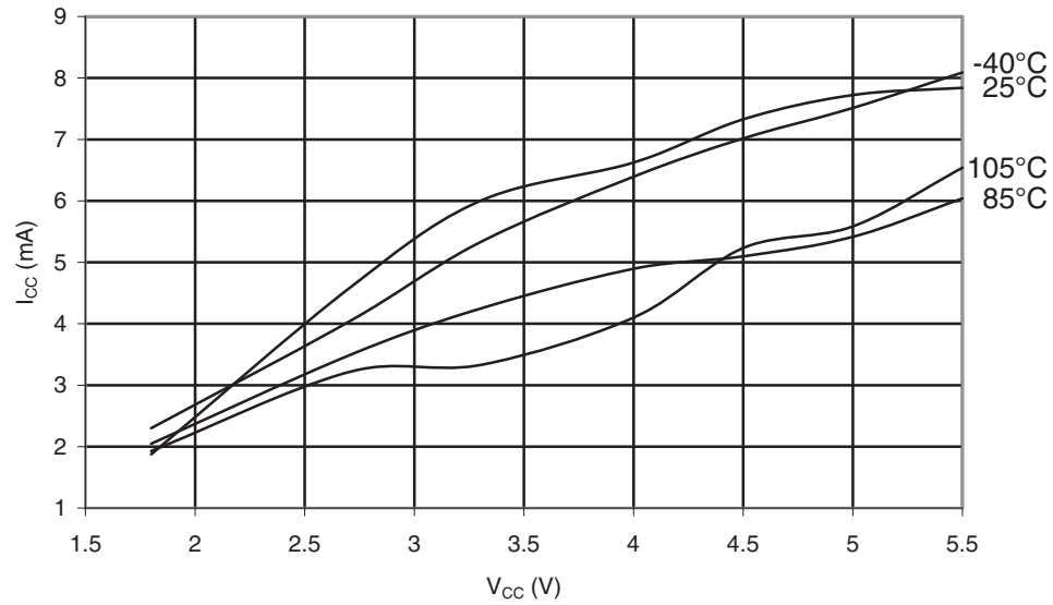
Figure 30-281. ATmega168PA: Programming Current vs. V_{CC}
