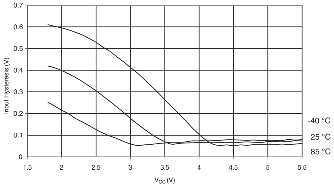
Figure 30-314. ATmega328: Reset Pin Input Hysteresis vs. V_{CC}
