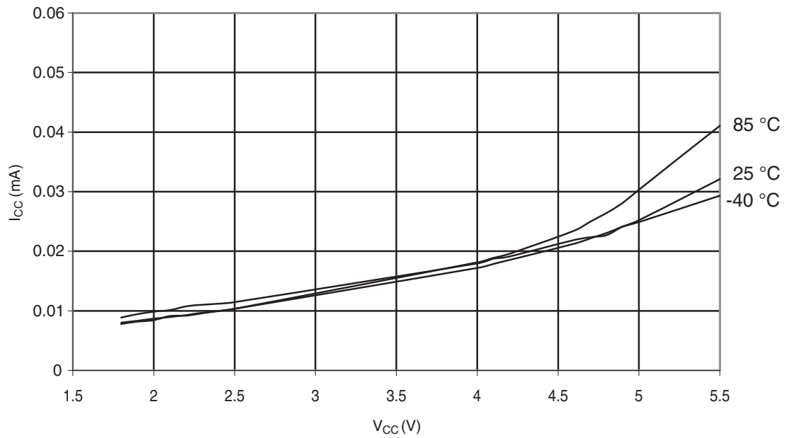
Figure 30-292. ATmega328: Idle Supply Current vs. V_{CC} (Internal RC Oscillator, 128kHz)
