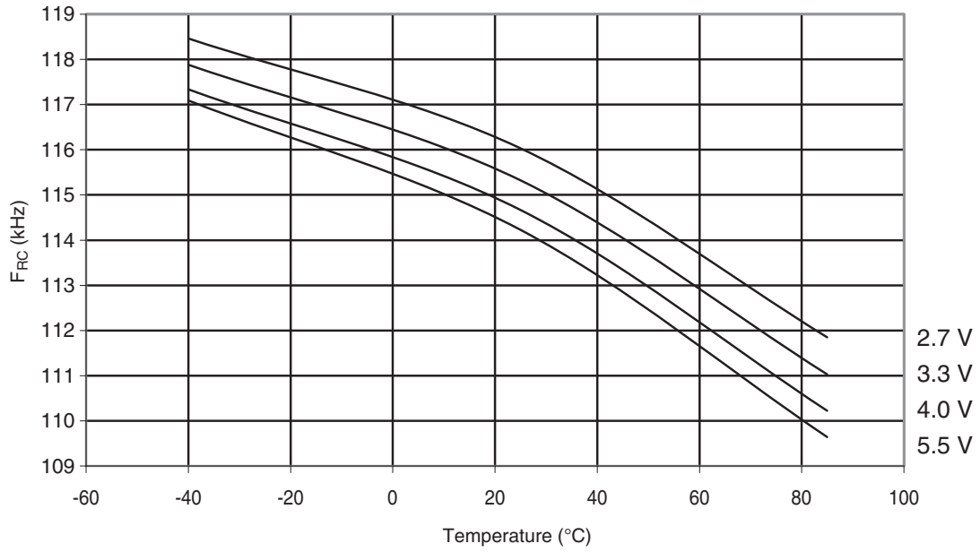
Figure 30-319. ATmega328: Watchdog Oscillator Frequency vs. Temperature
