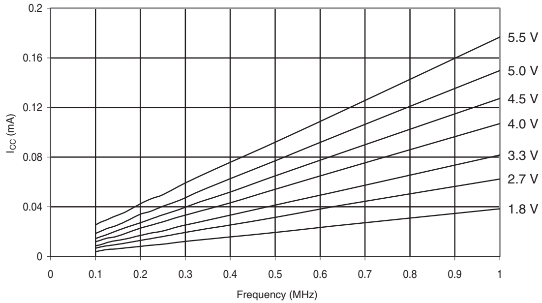
Figure 30-290. ATmega328: Idle Supply Current vs. Low Frequency (0.1-1.0MHz)
