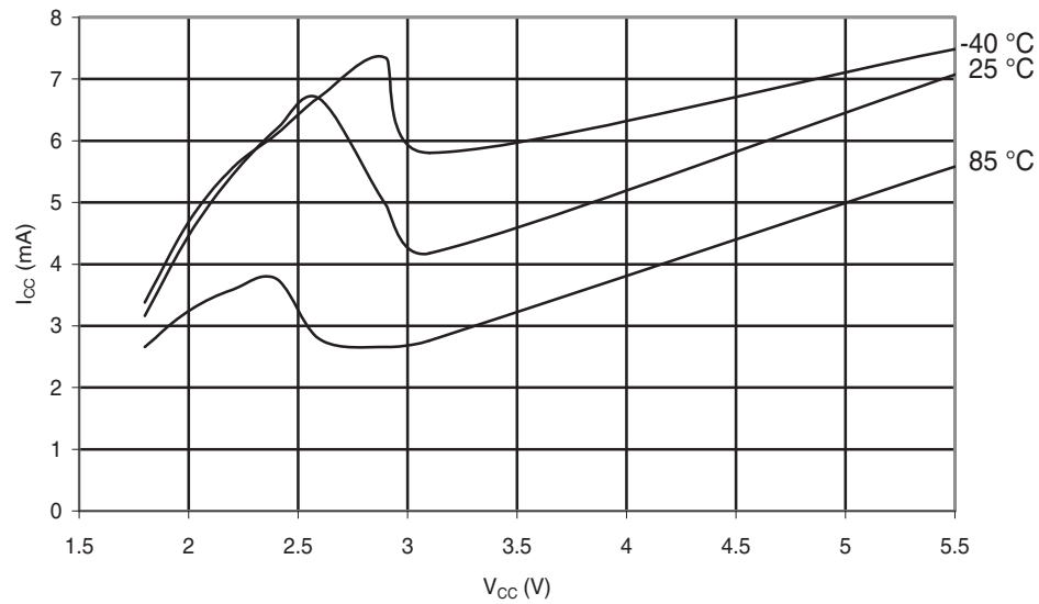
Figure 30-138. ATmega88A: Programming Current vs. V_{CC}
