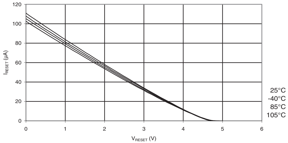
Figure 30-161. ATmega88PA: Reset Pull-up Resistor Current vs. Reset Pin Voltage ( V_{CC} = 5V )
