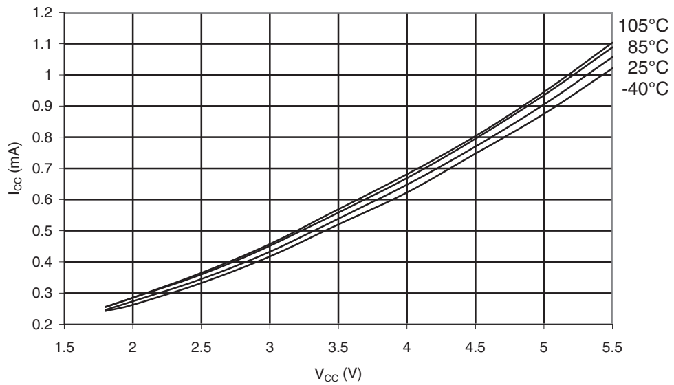
Figure 30-240. ATmega168PA: Active Supply Current vs. V_{CC} (Internal RC Oscillator, 1MHz)
