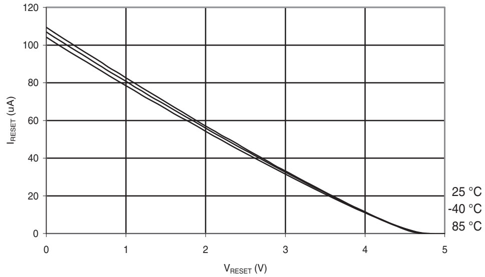
Figure 30-209. ATmega168A: Reset Pull-up Resistor Current vs. Reset Pin Voltage ( V_{CC} = 5\text{ V} )
