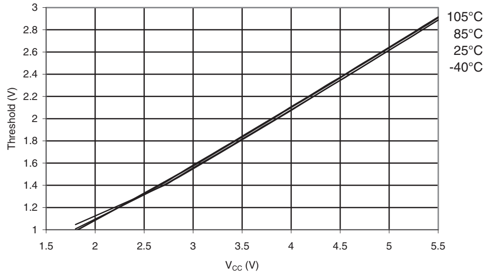
Figure 30-261. ATmega168PA I/O Pin Input Threshold Voltage vs. V_{CC} ( V_{IH} , I/O Pin read as '1')
