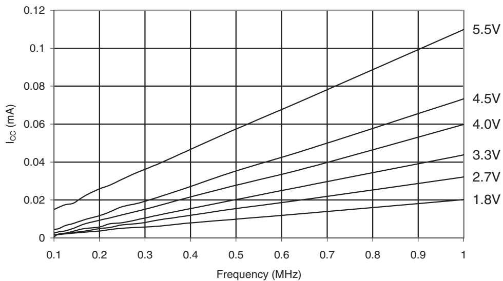
Figure 30-282. ATmega168PA: Reset Supply Current vs. Low Frequency (0.1MHz - 1.0MHz)
