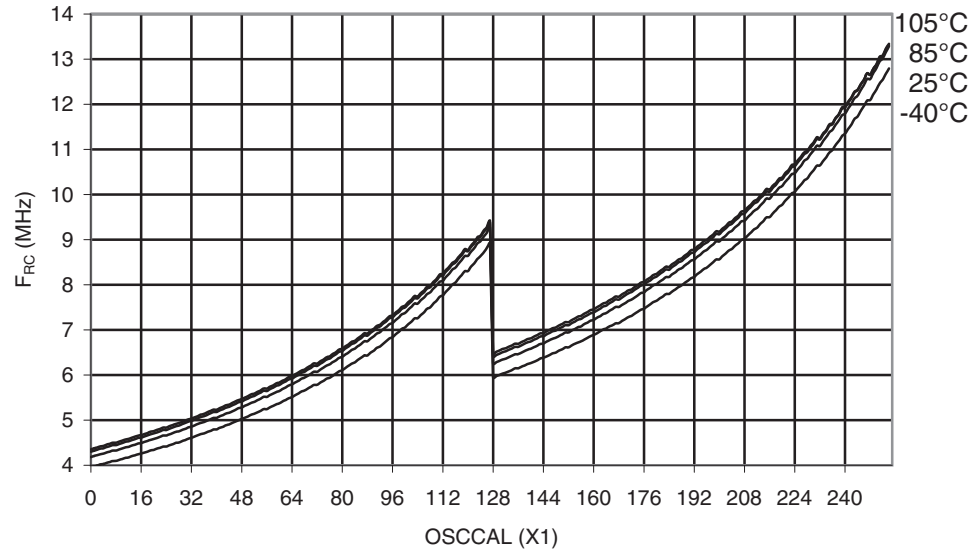
Figure 30-370. ATmega328P Calibrated 8MHz RC Oscillator Frequency vs. OSCCAL Value
