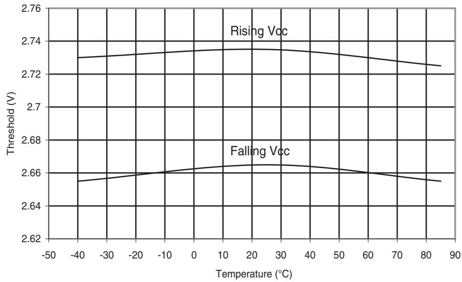
Figure 30-221. ATmega168A: BOD Thresholds vs. Temperature (BODLEVEL is 2.7 V)
