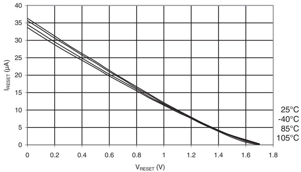
Figure 30-349. ATmega328P: Reset Pull-up Resistor Current vs. Reset Pin Voltage ( V_{CC} = 1.8V )
