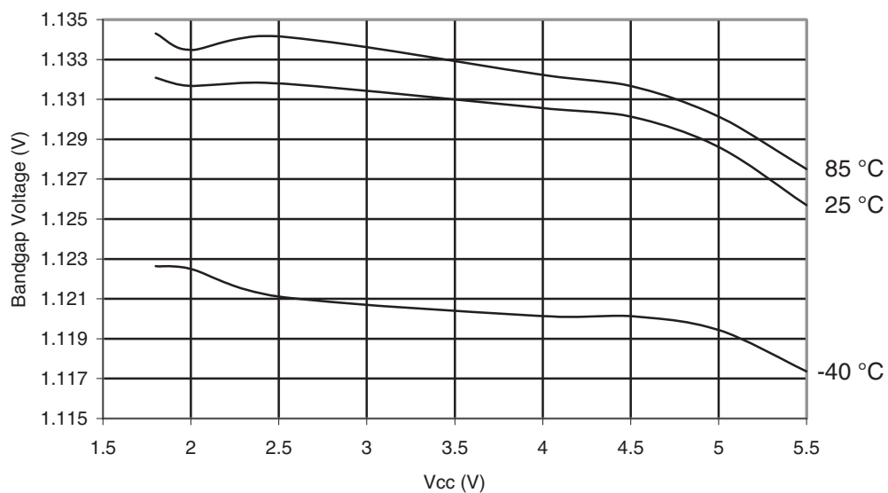
Figure 30-223. ATmega168A: Bandgap Voltage vs. V CC
