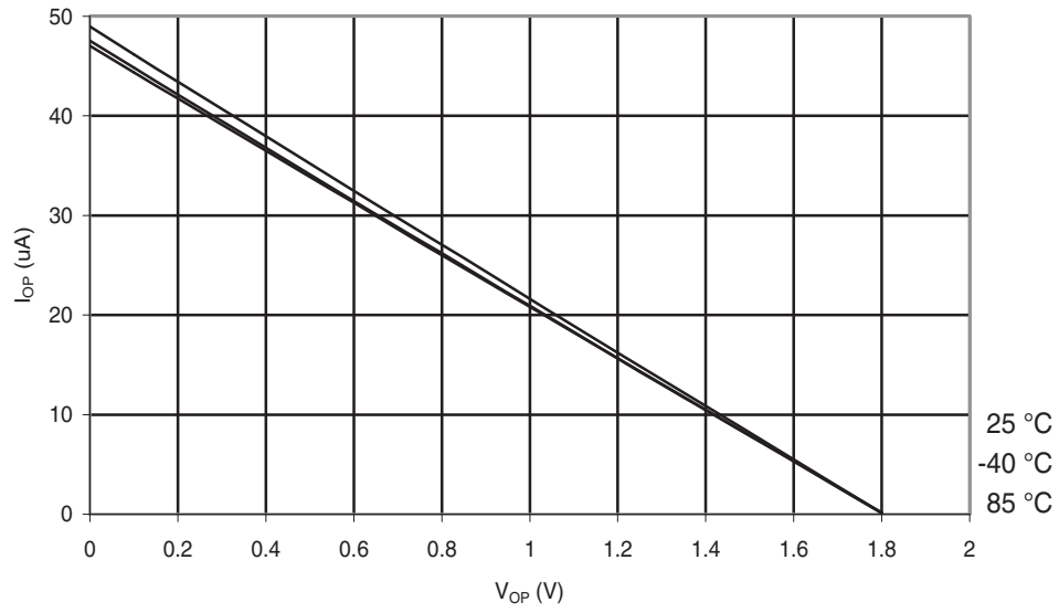
Figure 30-204. ATmega168A: I/O Pin Pull-up Resistor Current vs. Input Voltage ( V_{CC} = 1.8\text{ V} )
