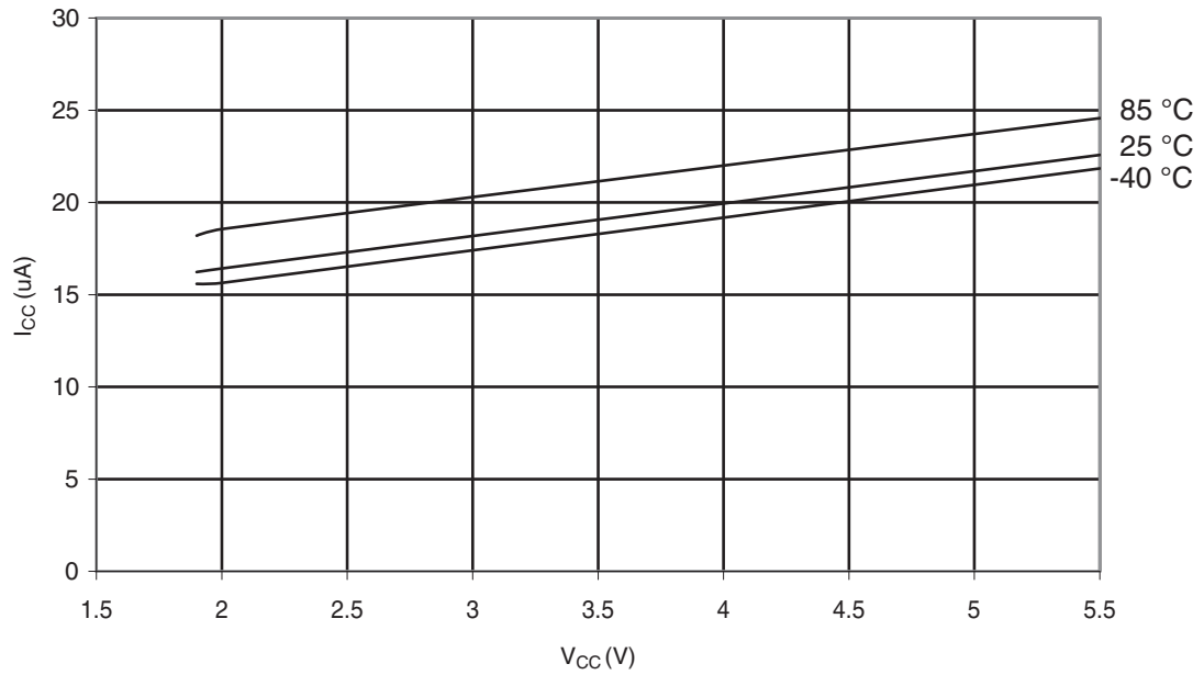
Figure 30-327. ATmega328: Brownout Detector Current vs. V_{CC}
