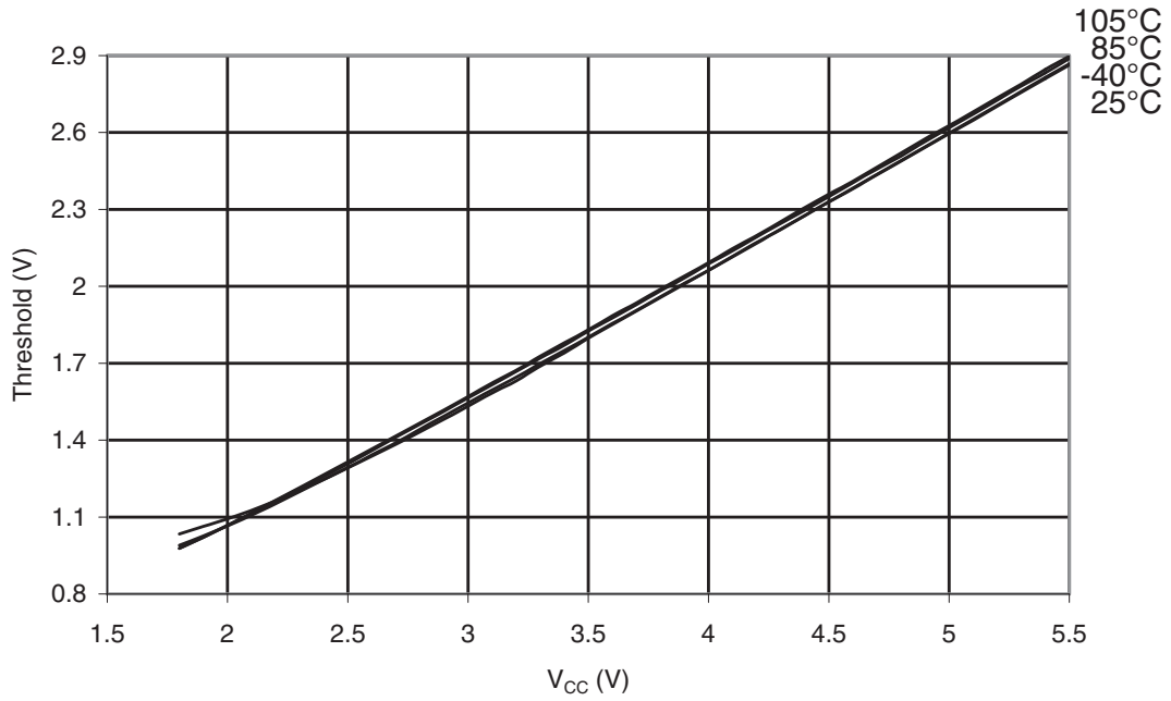
Figure 30-72. ATmega48PA: I/O Pin Input Threshold Voltage vs. V_{CC} ( V_{IH} , I/O Pin read as '1')
