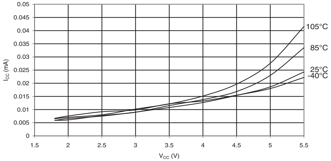
Figure 30-149. ATmega88PA: Idle Supply Current vs. V_{CC} (Internal RC Oscillator, 128kHz)
