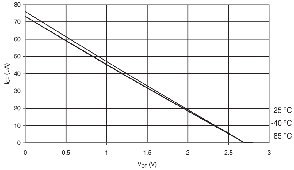
Figure 30-205. ATmega168A: I/O Pin Pull-up Resistor Current vs. Input Voltage ( V_{CC} = 2.7\text{ V} )
