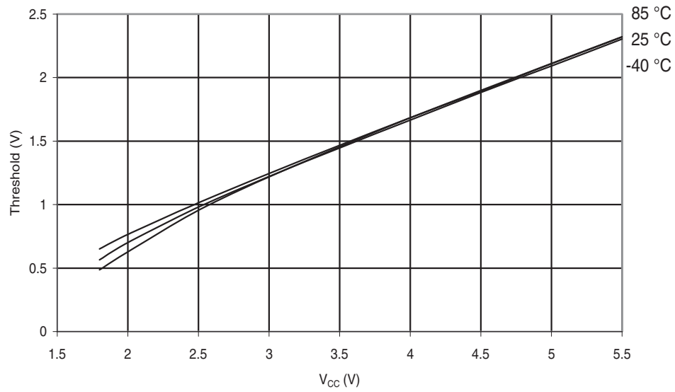
Figure 30-215. ATmega168A: I/O Pin Input Threshold Voltage vs. V_{CC} ( V_{IL} , I/O Pin read as '0')
