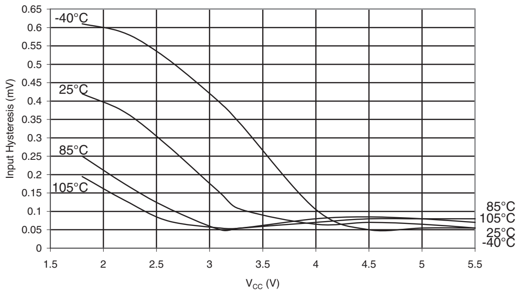
Figure 30-77. ATmega48PA: Reset Pin Input Hysteresis vs. V_{CC}
