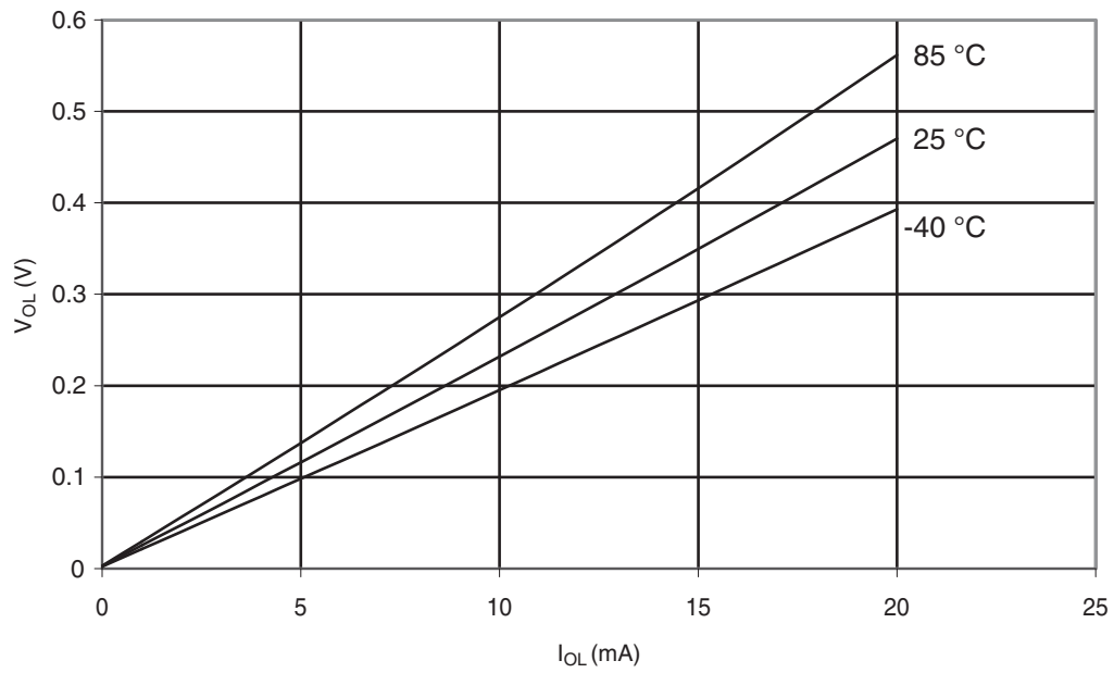
Figure 30-306. ATmega328: I/O Pin Output Voltage vs. Sink Current ( V_{CC} = 5\text{ V} )
