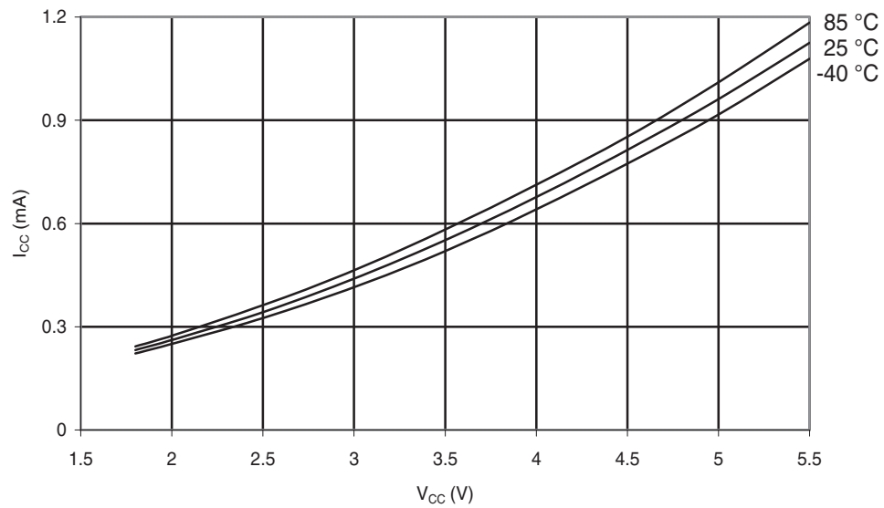
Figure 30-199. ATmega168A: Idle Supply Current vs. V_{CC} (Internal RC Oscillator, 8MHz)
