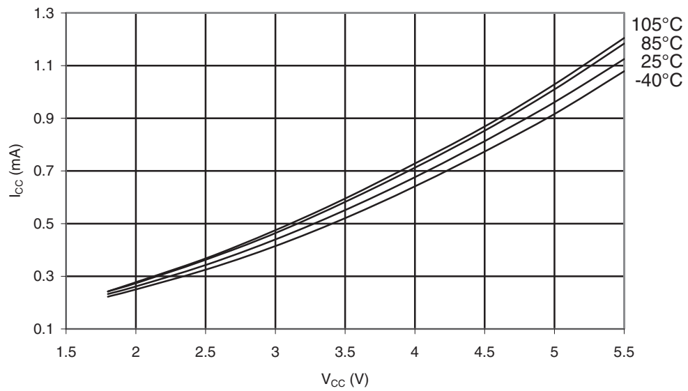
Figure 30-246. ATmega168PA: Idle Supply Current vs. V_{CC} (Internal RC Oscillator, 8MHz)
