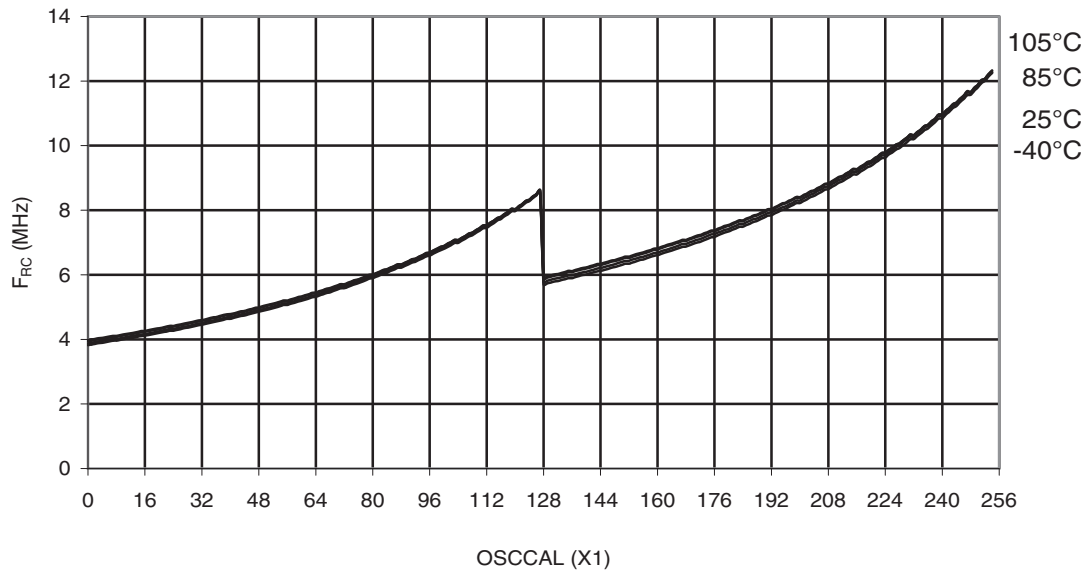
Figure 30-181. ATmega88PA: Calibrated 8MHz RC Oscillator Frequency vs. OSCCAL Value
