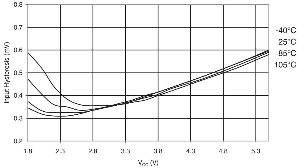
Figure 30-358. ATmega328P: I/O Pin Input Hysteresis vs. V_{CC}
