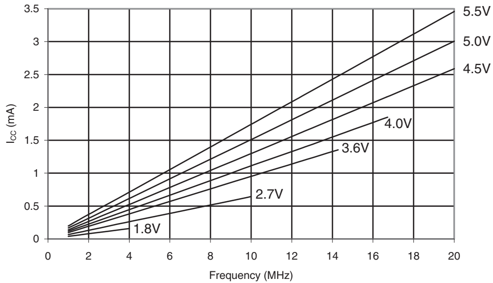
Figure 30-333. ATmega328P: Active Supply Current vs. Frequency (1-20MHz)
