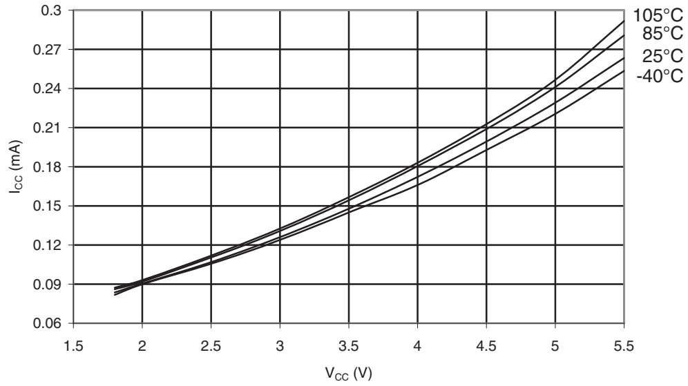
Figure 30-245. ATmega168PA: Idle Supply Current vs. V_{CC} (Internal RC Oscillator, 1MHz)
