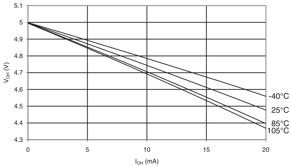
Figure 30-355. ATmega328P: I/O Pin Output Voltage vs. Source Current ( V_{CC} = 5V )
