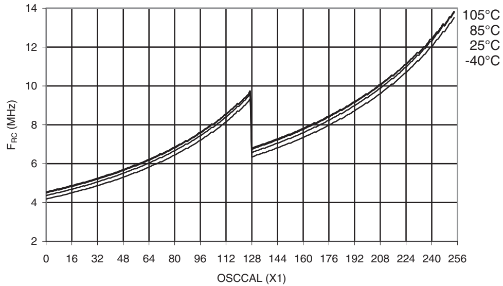
Figure 30-276. ATmega168PA: Calibrated 8MHz RC Oscillator Frequency vs. OSCCAL Value
