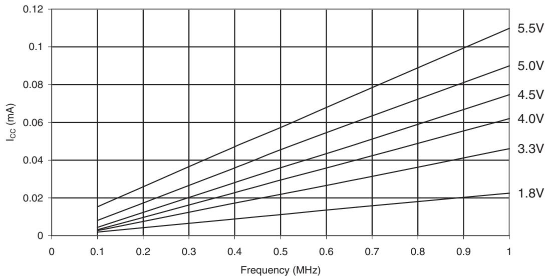
Figure 30-187. ATmega88PA: Reset Supply Current vs. Low Frequency (0.1MHz - 1.0MHz)
