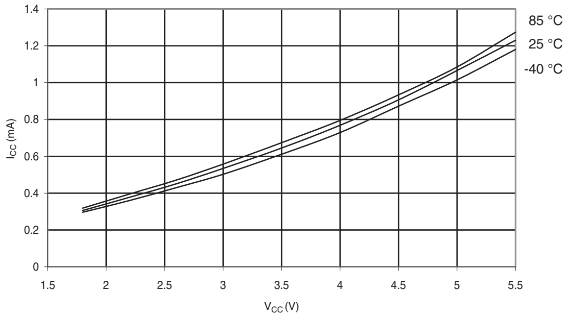
Figure 30-288. ATmega328: Active Supply Current vs. V_{CC} (Internal RC Oscillator, 1MHz)
