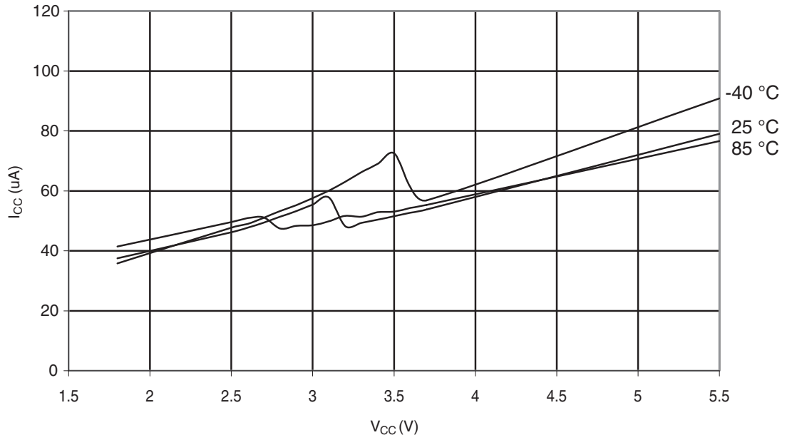
Figure 30-325. ATmega328: Analog Comparator Current vs. V_{CC}
