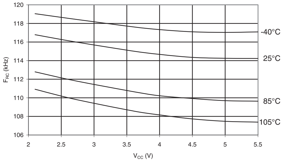
Figure 30-367. ATmega328P: Watchdog Oscillator Frequency vs. V_{CC}
