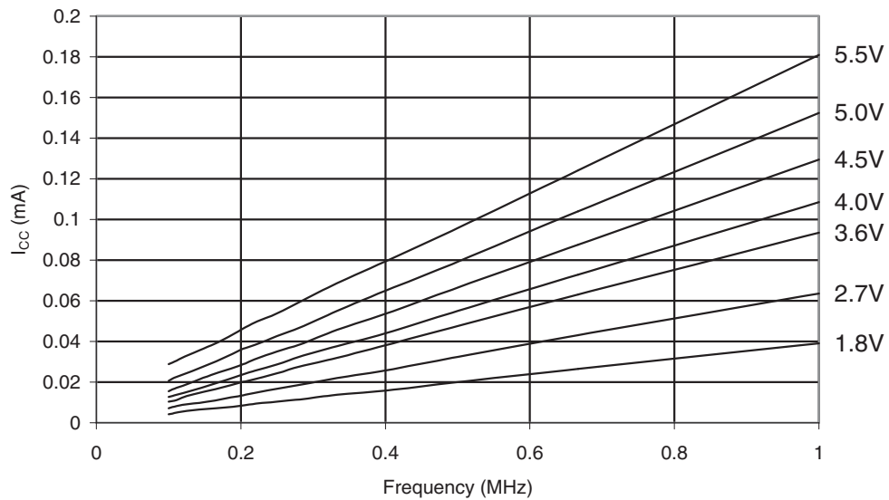
Figure 30-337. ATmega328P: Idle Supply Current vs. Low Frequency (0.1-1.0MHz)
