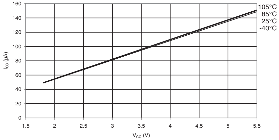
Figure 30-185. ATmega88PA: Brownout Detector Current vs. V_{CC}
