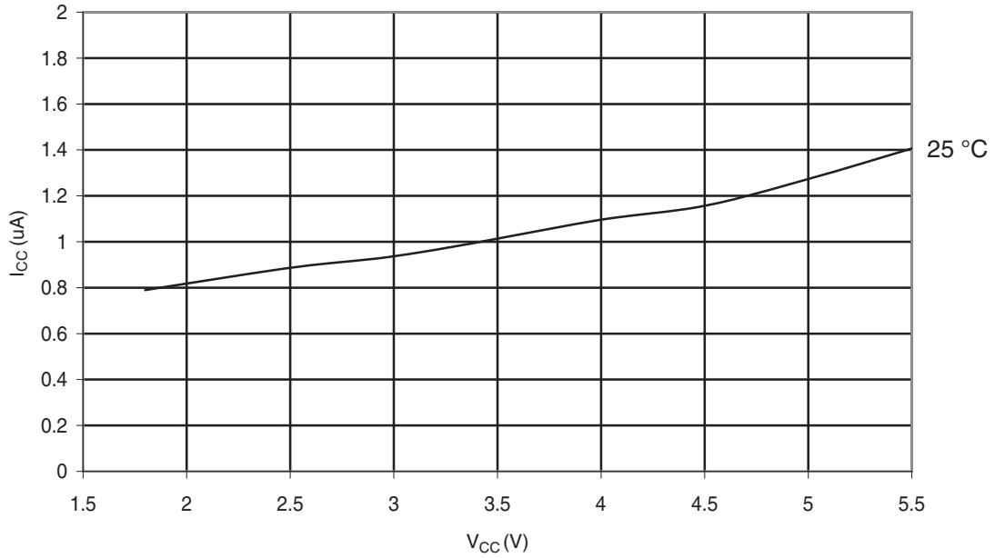
Figure 30-297. ATmega328: Power-Save Supply Current vs. V_{CC} (Watchdog Timer Disabled and 32kHz Crystal Oscillator Running)
