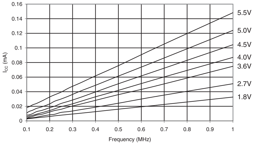
Figure 30-376. ATmega328P: Reset Supply Current vs. Low Frequency (0.1MHz - 1.0MHz)
