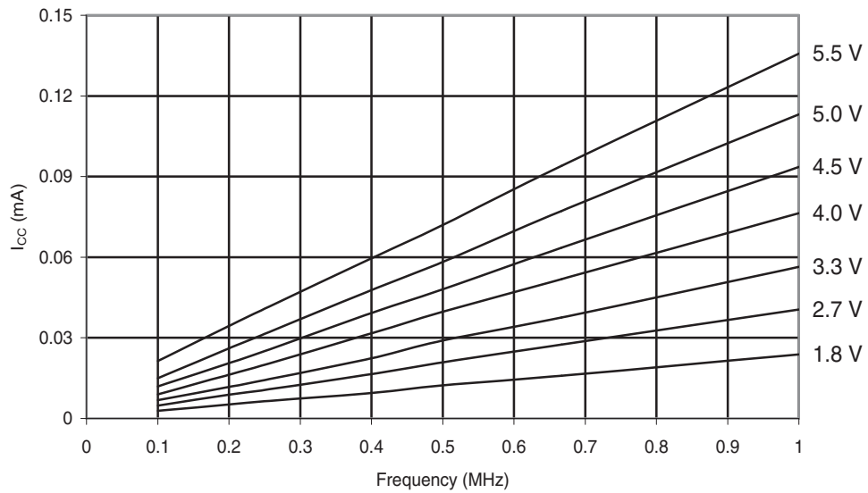
Figure 30-195. ATmega168A: Idle Supply Current vs. Low Frequency (0.1-1.0MHz)
