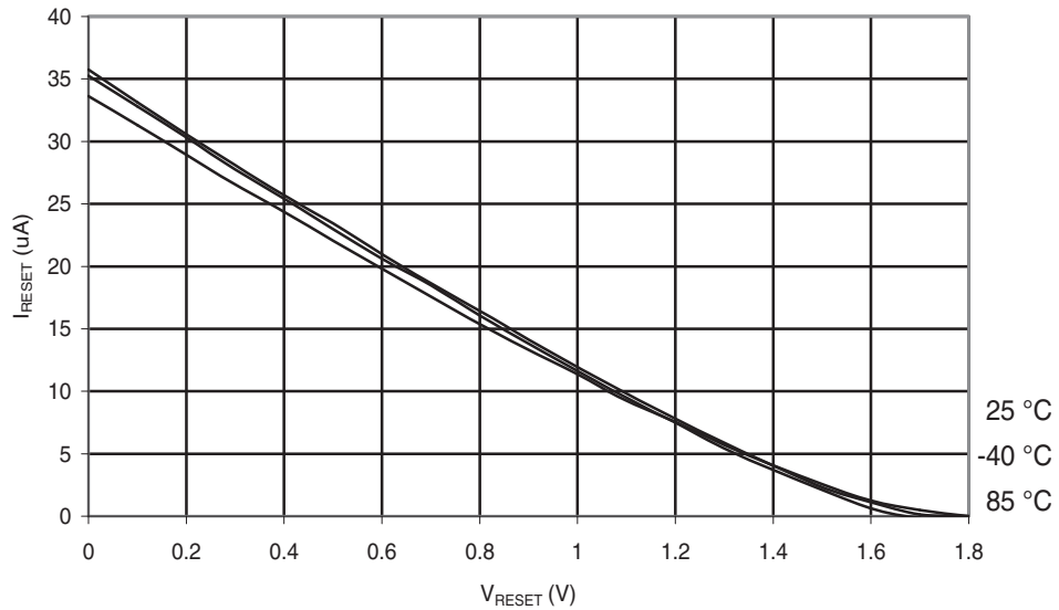
Figure 30-207. ATmega168A: Reset Pull-up Resistor Current vs. Reset Pin Voltage ( V_{CC} = 1.8\text{ V} )
