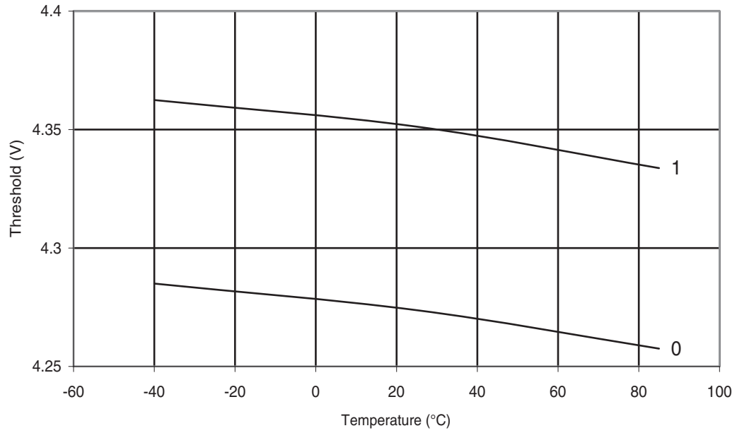
Figure 30-317. ATmega328: BOD Thresholds vs. Temperature (BODLEVEL is 4.3 V)
