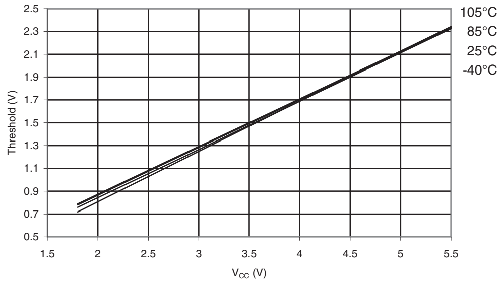
Figure 30-360. ATmega328P: Reset Input Threshold Voltage vs. V_{CC} ( V_{IL} , I/O Pin read as '0')
