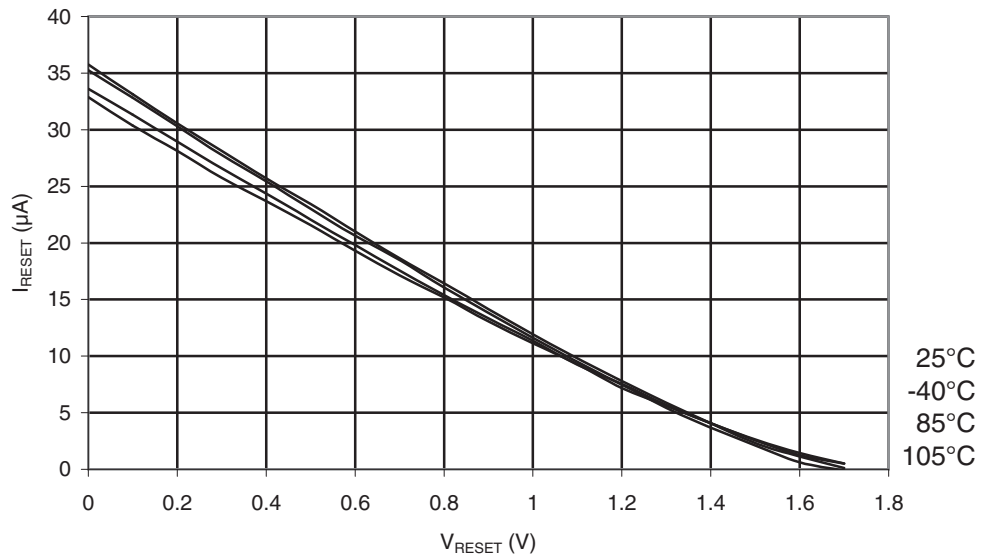
Figure 30-254. ATmega168PA: Reset Pull-up Resistor Current vs. Reset Pin Voltage ( V_{CC} = 1.8V )
