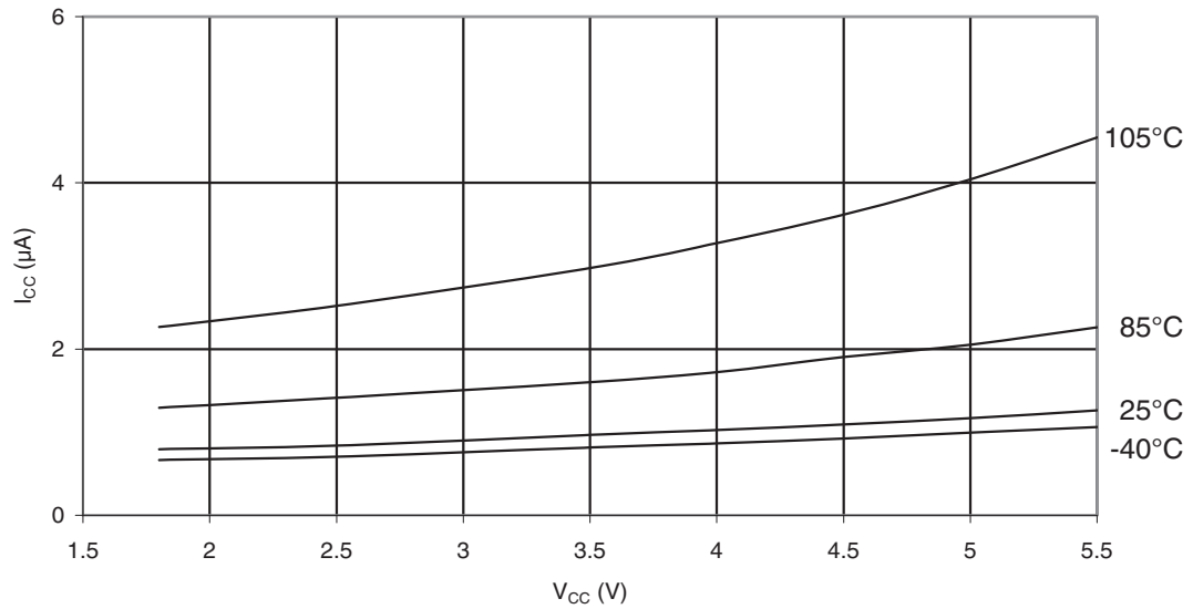
Figure 30-154. ATmega88PA: Power-Save Supply Current vs. V_{CC} (Watchdog Timer Disabled and 32kHz Crystal Oscillator Running)
