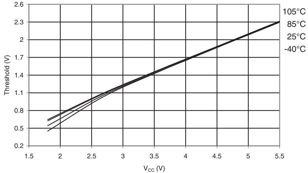
Figure 30-357. ATmega328P: I/O Pin Input Threshold Voltage vs. V_{CC} ( V_{IL} , I/O Pin read as '0')
