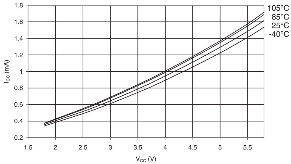
Figure 30-341. ATmega328P Idle Supply Current vs. V_{CC} (Internal RC Oscillator, 8MHz)
