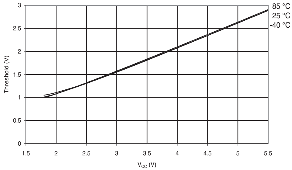
Figure 30-214. ATmega168A: I/O Pin Input Threshold Voltage vs. V_{CC} ( V_{IH} , I/O Pin read as '1')
