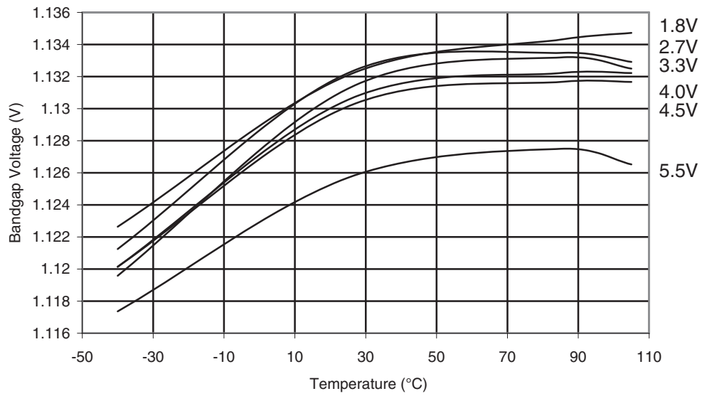
Figure 30-270. ATmega168PA: Calibrated Bandgap Voltage vs. Temperature
