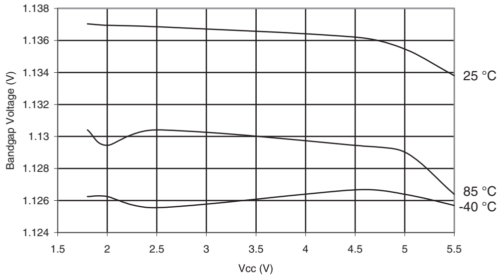
Figure 30-318. ATmega328: Bandgap Voltage vs. V_{CC}
