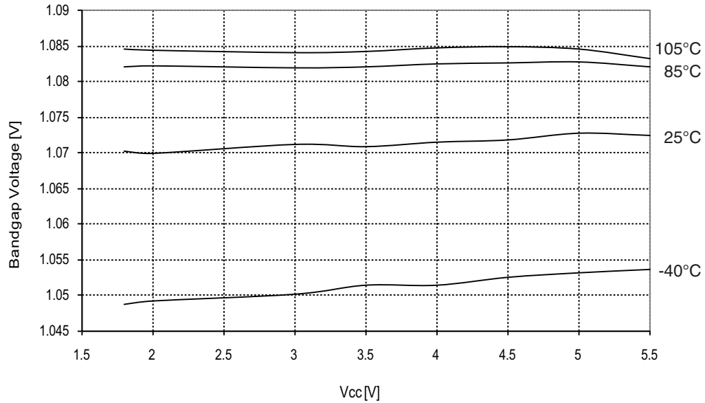
Figure 30-176. ATmega88PA: Bandgap Voltage vs. V_{CC}
