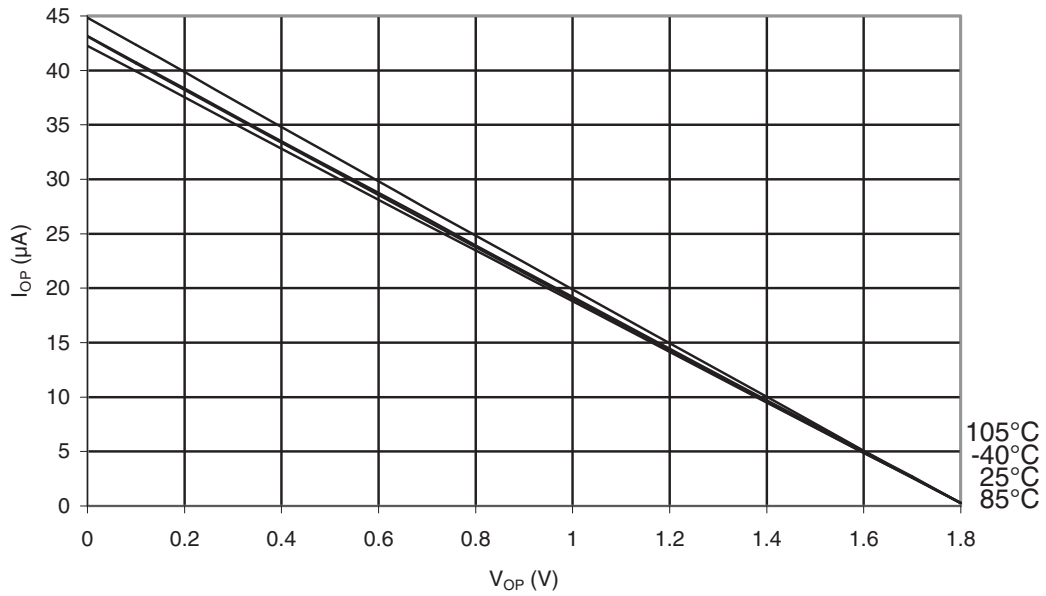
Figure 30-63. ATmega48PA: I/O Pin Pull-up Resistor Current vs. Input Voltage ( V_{CC} = 2.7V )
