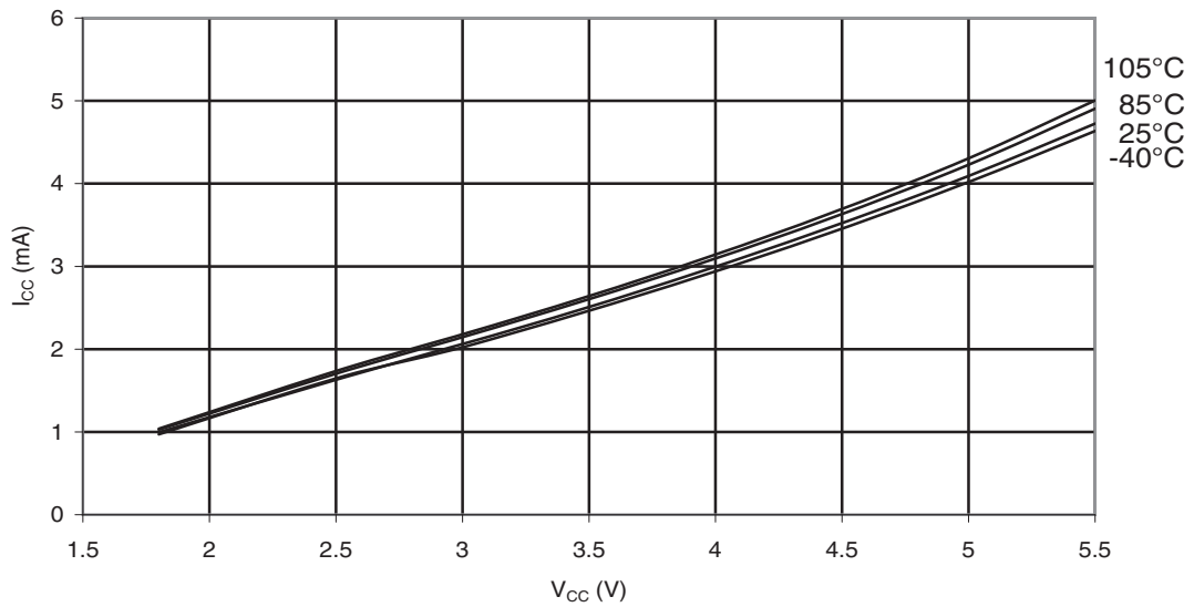
Figure 30-146. ATmega88PA: Active Supply Current vs. V_{CC} (Internal RC Oscillator, 8MHz)
