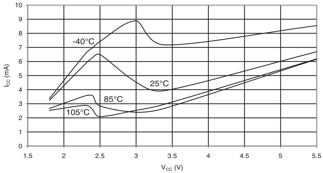
Figure 30-186. ATmega88PA: Programming Current vs. V_{CC}
