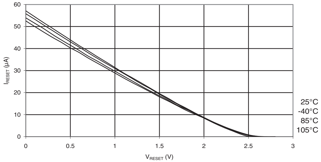
Figure 30-160. ATmega88PA: Reset Pull-up Resistor Current vs. Reset Pin Voltage ( V_{CC} = 2.7V )
