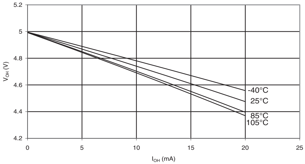
Figure 30-165. ATmega88PA: I/O Pin Output Voltage vs. Source Current ( V_{CC} = 5V )
