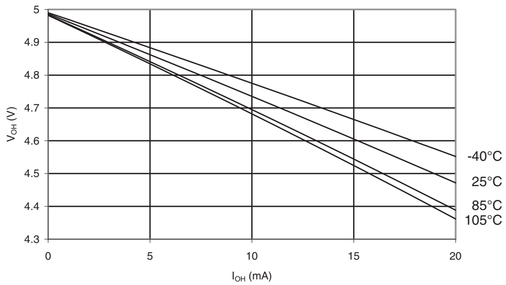
Figure 30-260. ATmega168PA I/O Pin Output Voltage vs. Source Current ( V_{CC} = 5V )
