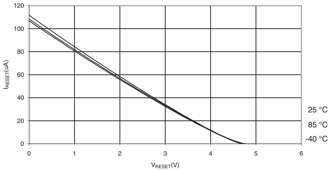
Figure 30-304. ATmega328: Reset Pull-up Resistor Current vs. Reset Pin Voltage ( V_{CC} = 5\text{ V} )
