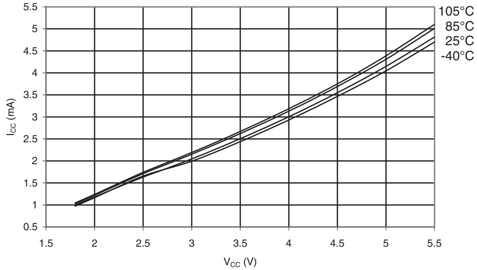
Figure 30-241. ATmega168PA: Active Supply Current vs. V_{CC} (Internal RC Oscillator, 8MHz)
