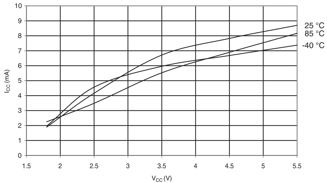
Figure 30-328. ATmega328: Programming Current vs. V_{CC}
