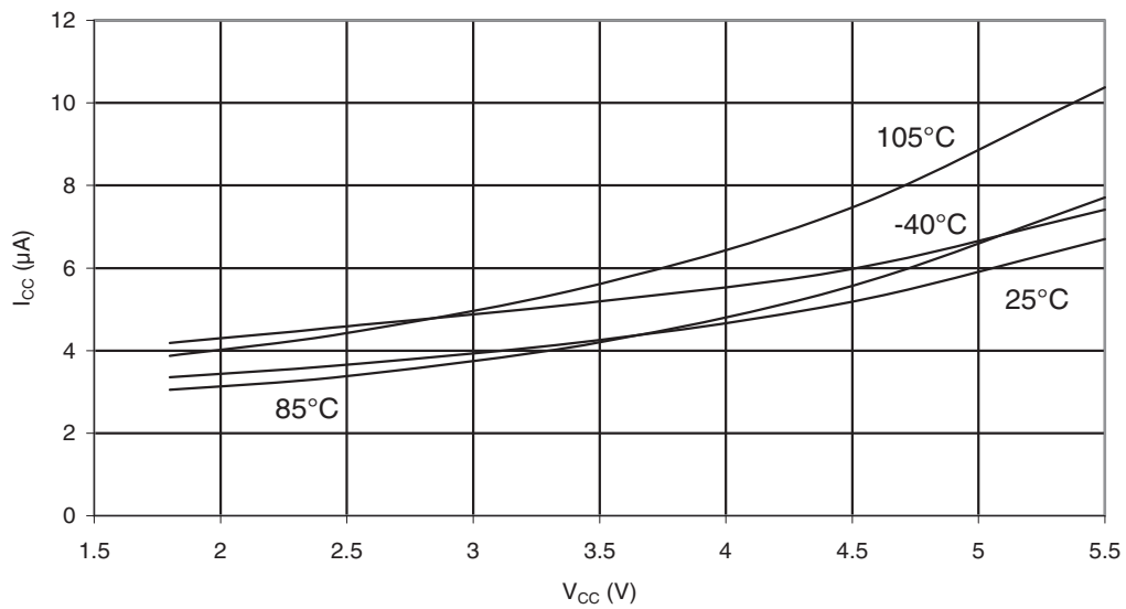
Figure 30-153. ATmega88PA: Power-Down Supply Current vs. V_{CC} (Watchdog Timer Enabled)
