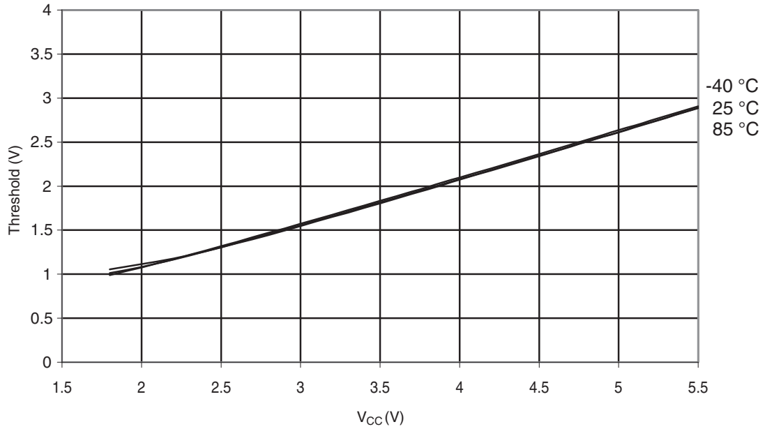
Figure 30-309. ATmega328: I/O Pin Input Threshold Voltage vs. V_{CC} ( V_{IH} , I/O Pin read as '1')
