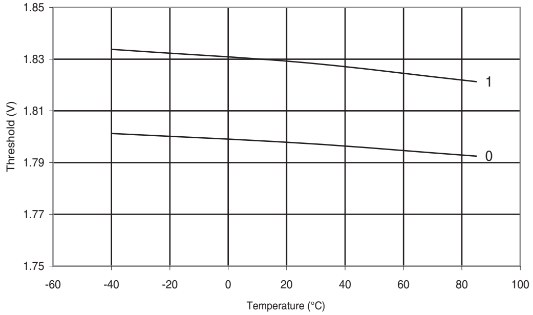
Figure 30-315. ATmega328: BOD Thresholds vs. Temperature (BODLEVEL is 1.8 V)
