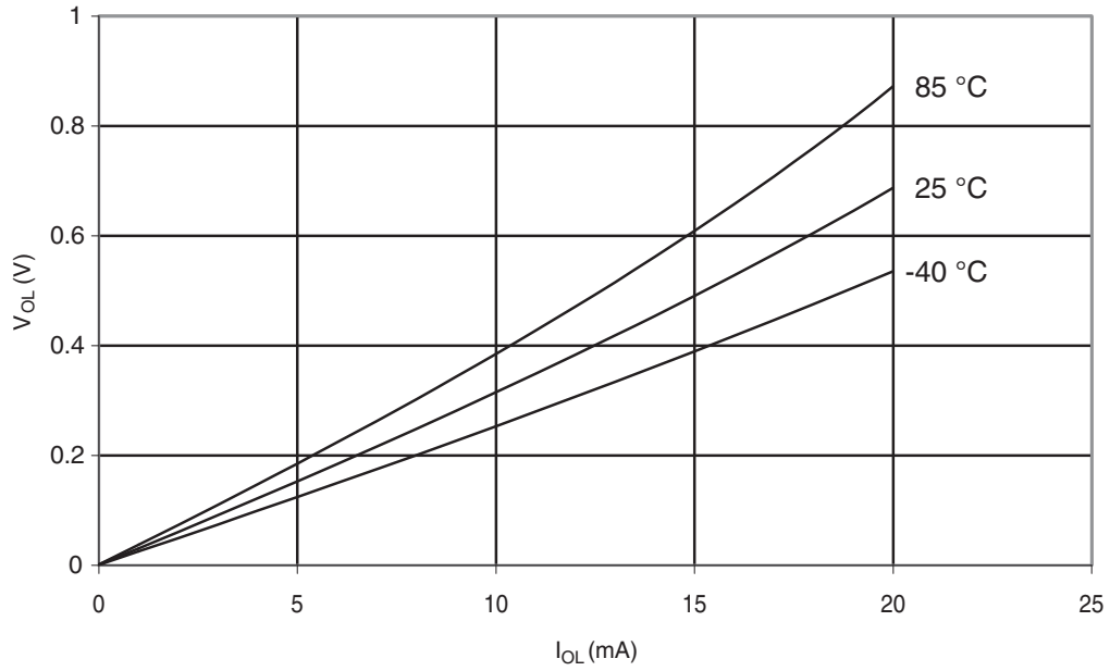
Figure 30-305. ATmega328: I/O Pin Output Voltage vs. Sink Current ( V_{CC} = 3\text{ V} )
