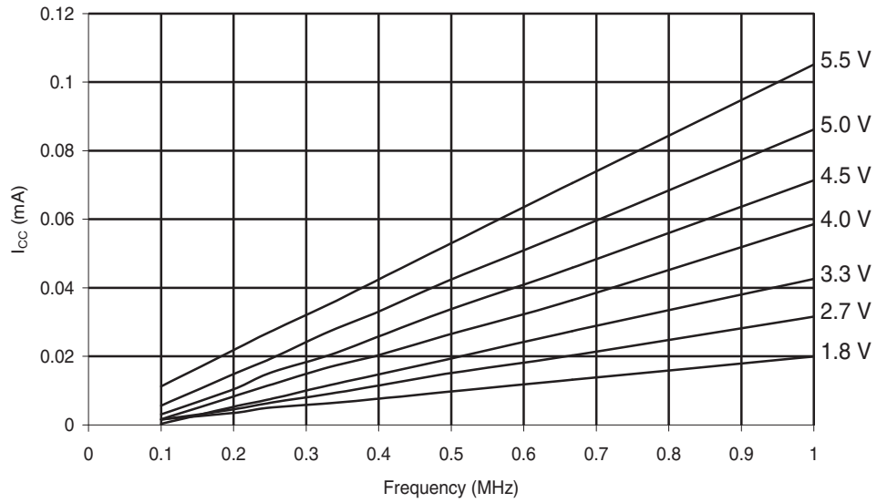
Figure 30-234. ATmega168A: Reset Supply Current vs. Low Frequency (0.1 - 1.0MHz)
