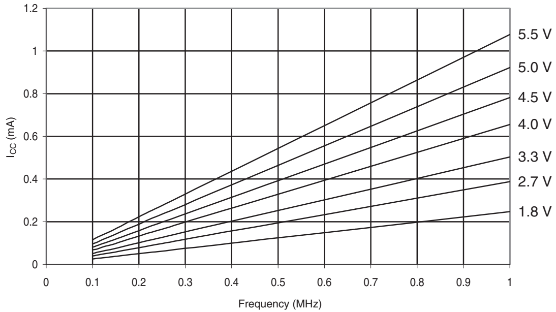
Figure 30-285. ATmega328: Active Supply Current vs. Low Frequency (0.1-1.0MHz)
