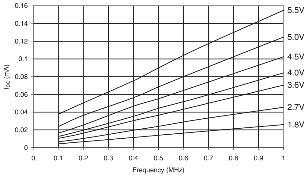
Figure 30-242. ATmega168PA: Idle Supply Current vs. Low Frequency (0.1-1.0MHz)
