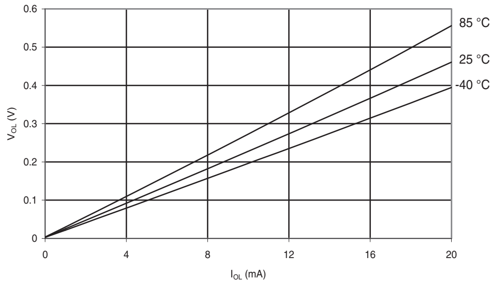
Figure 30-211. ATmega168A: I/O Pin Output Voltage vs. Sink Current ( V_{CC} = 5\text{ V} )
