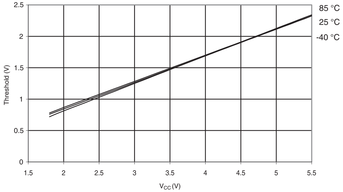
Figure 30-313. ATmega328: Reset Input Threshold Voltage vs. V_{CC} ( V_{IL} , I/O Pin read as '0')
