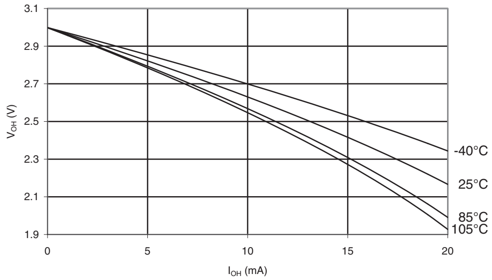
Figure 30-354. ATmega328P: I/O Pin Output Voltage vs. Source Current ( V_{CC} = 3V )
