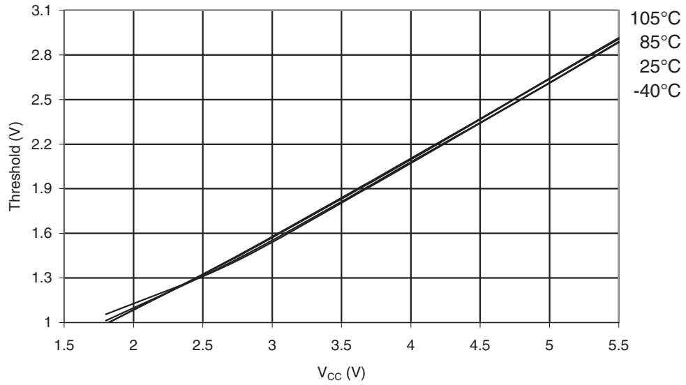
Figure 30-356. ATmega328P: I/O Pin Input Threshold Voltage vs. V_{CC} ( V_{IH} , I/O Pin read as '1')
