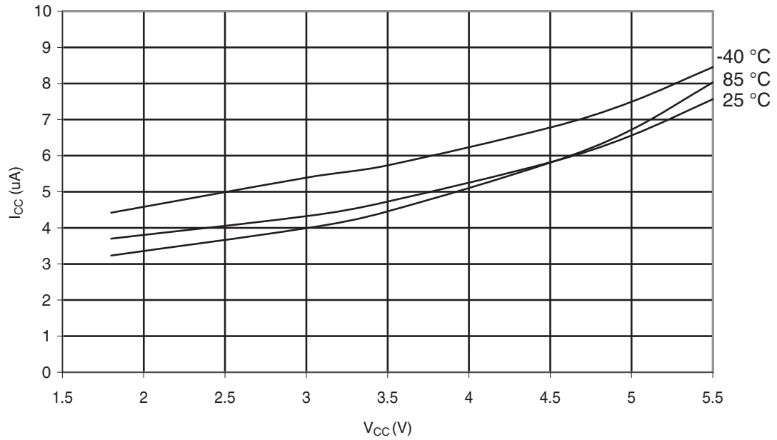
Figure 30-296. ATmega328: Power-Down Supply Current vs. V_{CC} (Watchdog Timer Enabled)
