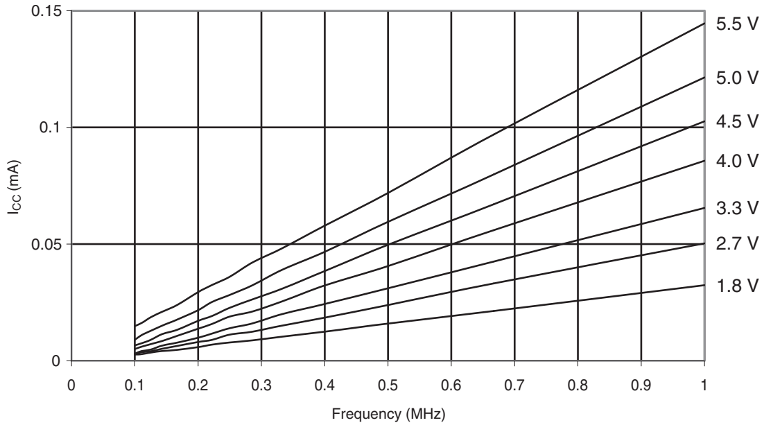
Figure 30-329. ATmega328: Reset Supply Current vs. Low Frequency (0.1 - 1.0MHz)
