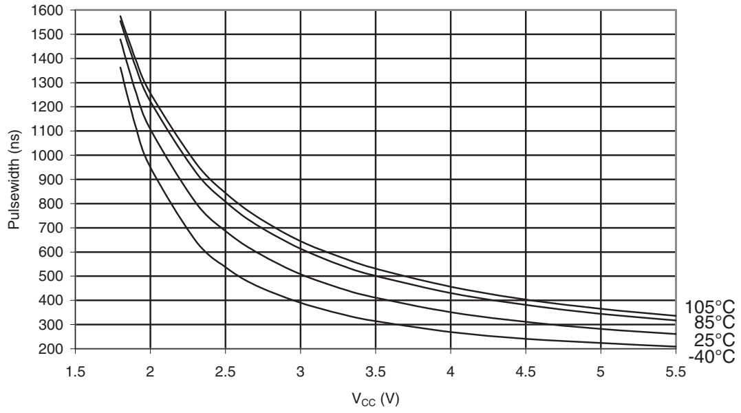
Figure 30-94. ATmega48PA: Minimum Reset Pulse width vs. V_{CC}
