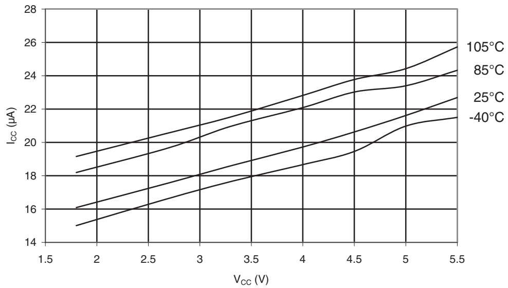
Figure 30-280. ATmega168PA: Brownout Detector Current vs. V_{CC}
