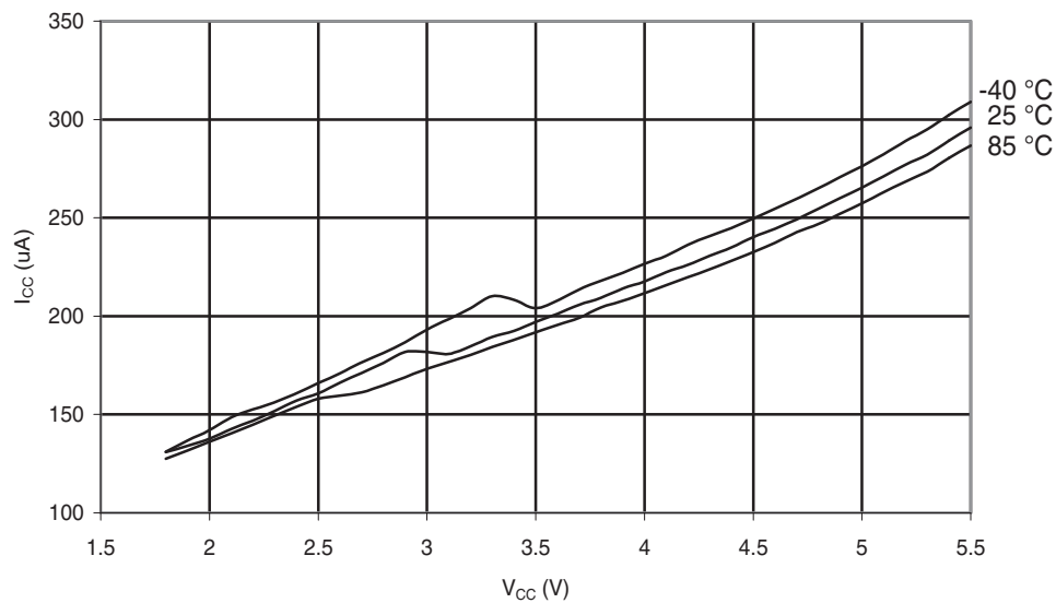
Figure 30-229. ATmega168A: ADC Current vs. V_{CC} (AREF = AV_{CC} )
