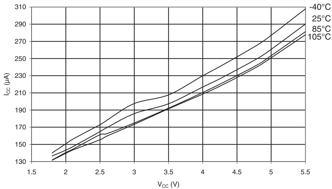
Figure 30-87. ATmega48PA: ADC Current vs. V_{CC} (AREF = AV_{CC} )
