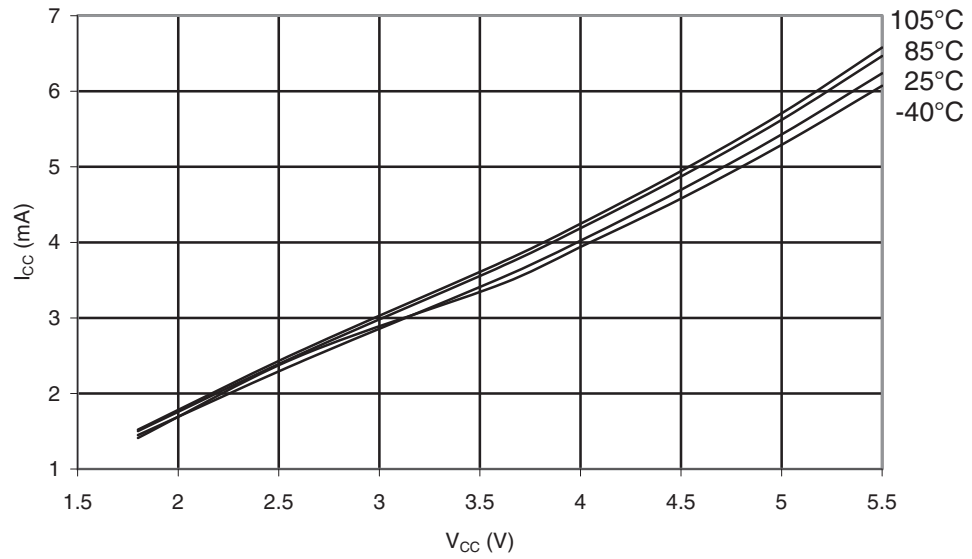
Figure 30-336. ATmega328P: Active Supply Current vs. V_{CC} (Internal RC Oscillator, 8MHz)
