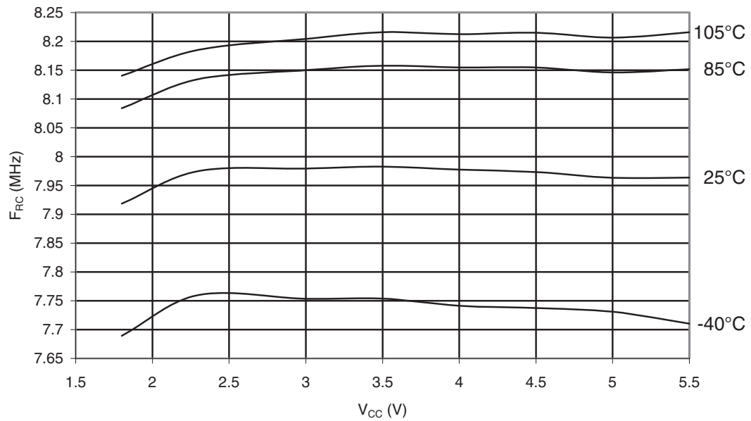
Figure 30-84. ATmega48PA: Calibrated 8MHz RC Oscillator Frequency vs. V_{CC}
