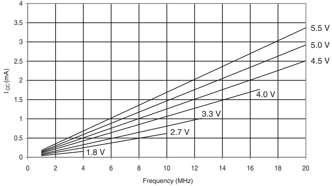
Figure 30-291. ATmega328: Idle Supply Current vs. Frequency (1-20MHz)
