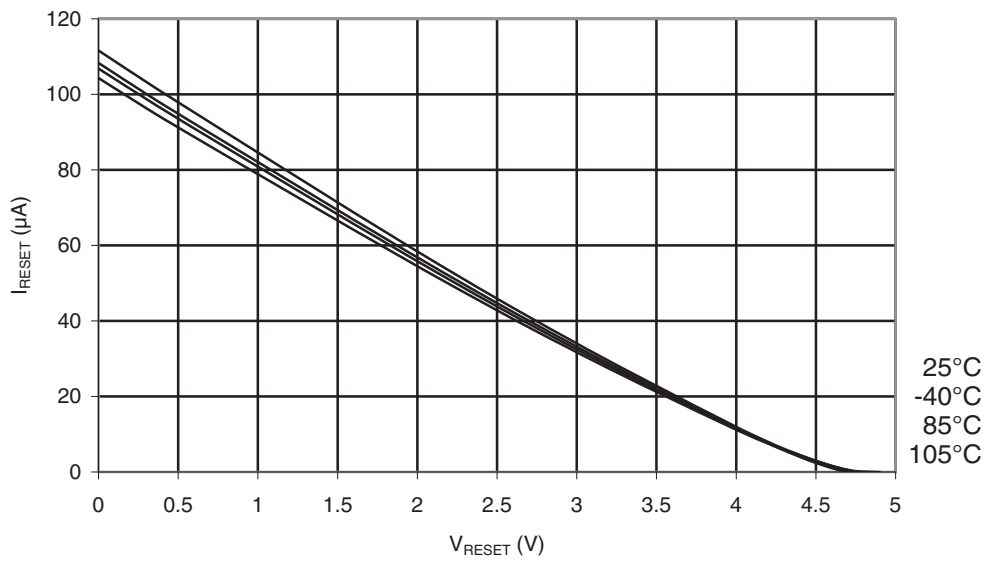
Figure 30-351. ATmega328P: Reset Pull-up Resistor Current vs. Reset Pin Voltage ( V_{CC} = 5V )
