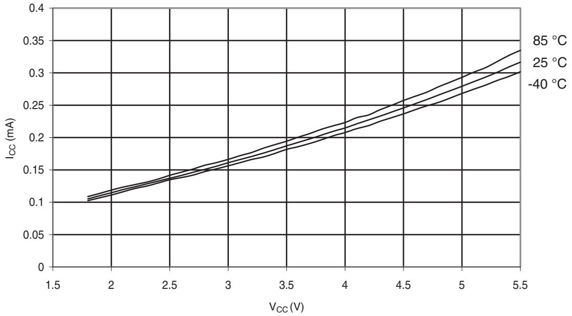
Figure 30-293. ATmega328: Idle Supply Current vs. V_{CC} (Internal RC Oscillator, 1MHz)
