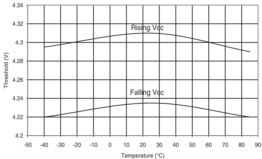
Figure 30-222. ATmega168A: BOD Thresholds vs. Temperature (BODLEVEL is 4.3 V)
