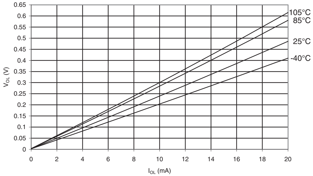
Figure 30-69. ATmega48PA: I/O Pin Output Voltage vs. Sink Current ( V_{CC} = 5V )
