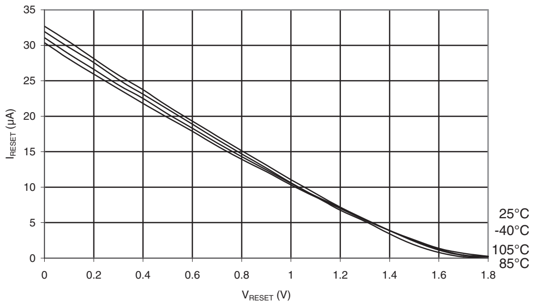
Figure 30-65. ATmega48PA: Reset Pull-up Resistor Current vs. Reset Pin Voltage ( V_{CC} = 1.8V )
