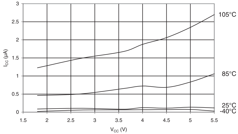
Figure 30-342. ATmega328P: Power-Down Supply Current vs. V_{CC} (Watchdog Timer Disabled)
