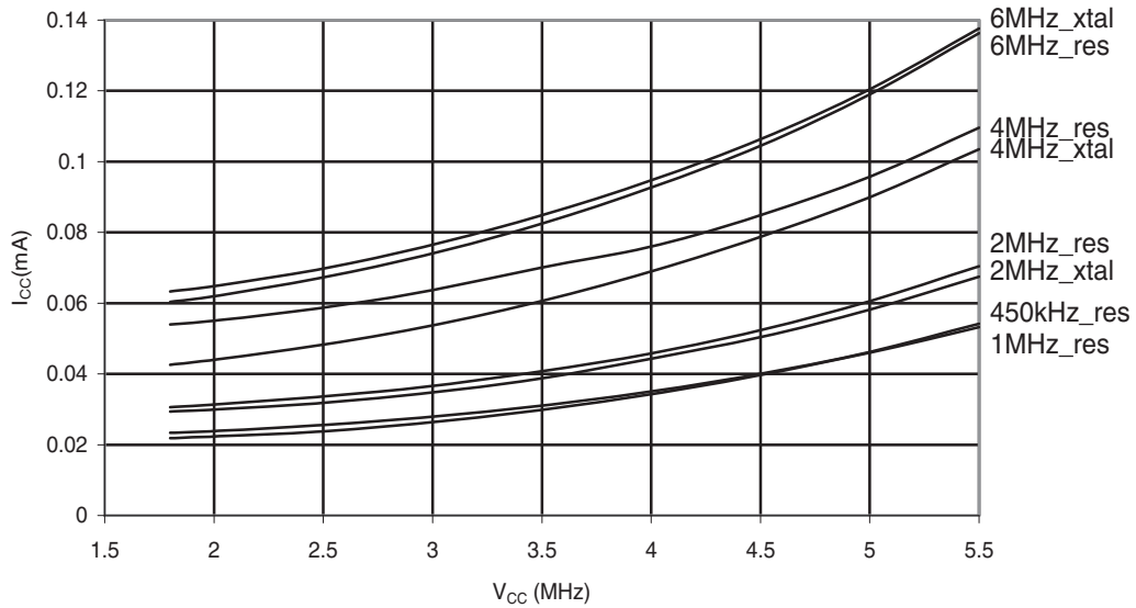
Figure 30-203. ATmega168A: Standby Supply Current vs. V_{CC} (Watchdog Timer Disabled)
