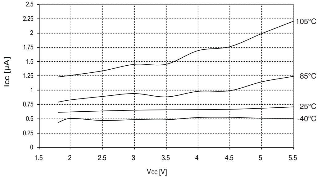
Figure 30-60. ATmega48PA: Power-Save Supply Current vs. V_{CC} (Watchdog Timer Disabled and 32kHz Crystal Oscillator Running)
