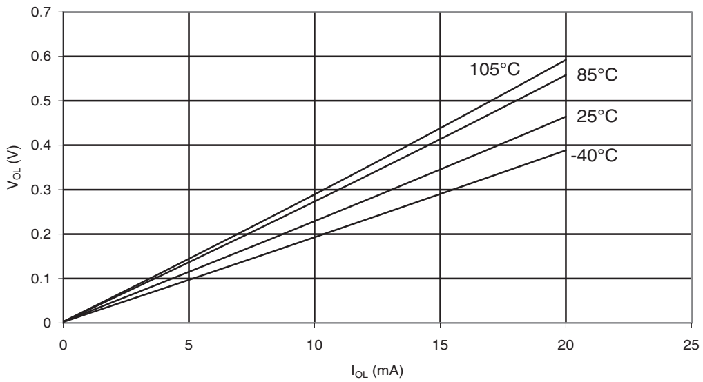
Figure 30-163. ATmega88PA: I/O Pin Output Voltage vs. Sink Current ( V_{CC} = 5V )
