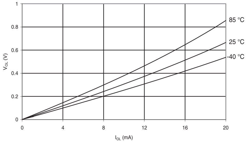
Figure 30-210. ATmega168A: I/O Pin Output Voltage vs. Sink Current ( V_{CC} = 3\text{ V} )
