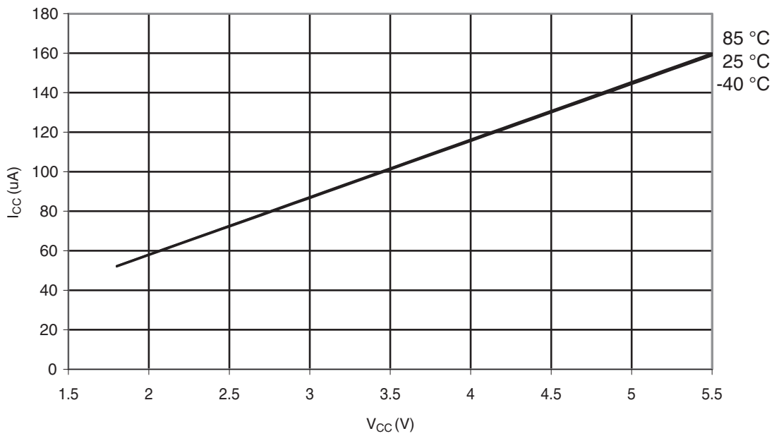
Figure 30-326. ATmega328: AREF External Reference Current vs. V_{CC}
