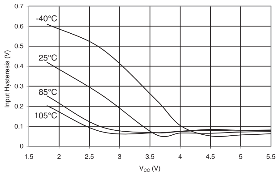
Figure 30-361. ATmega328P: Reset Pin Input Hysteresis vs. V_{CC}
