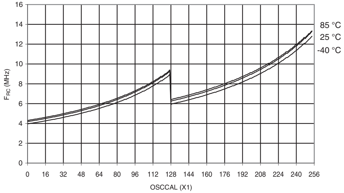
Figure 30-323. ATmega328: Calibrated 8MHz RC Oscillator Frequency vs. OSCCAL Value
