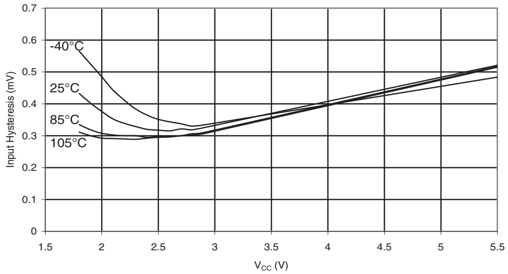
Figure 30-168. ATmega88PA: I/O Pin Input Hysteresis vs. V_{CC}
