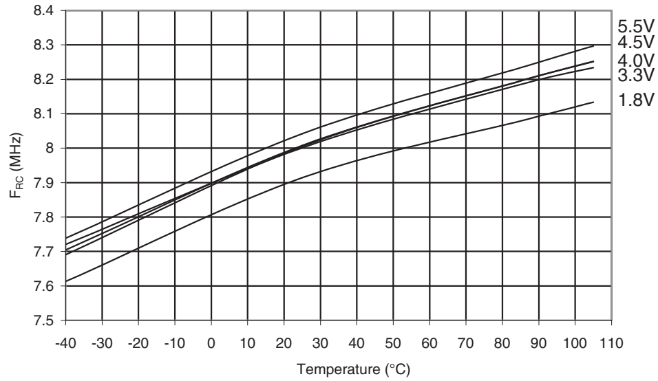
Figure 30-275. ATmega168PA: Calibrated 8MHz RC Oscillator Frequency vs. Temperature
