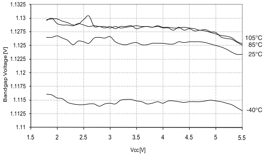
Figure 30-81. ATmega48PA: Bandgap Voltage vs. V_{CC}
