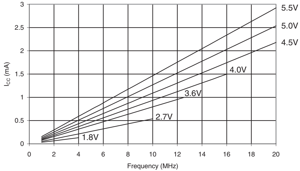
Figure 30-377. ATmega328P Reset Supply Current vs. Frequency (1MHz - 20MHz)
