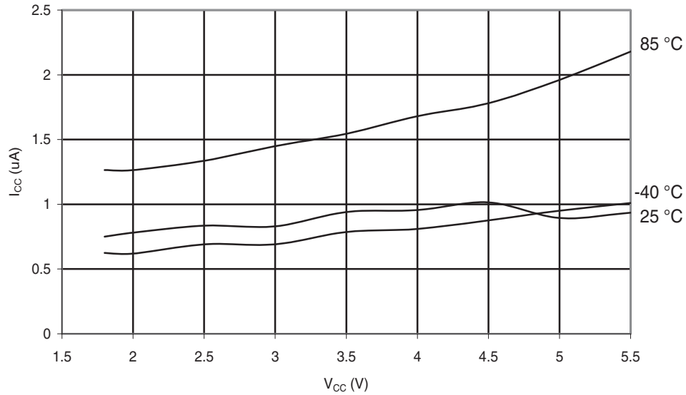
Figure 30-202. ATmega168A: Power-Save Supply Current vs. V_{CC} (Watchdog Timer Disabled and 32kHz Crystal Oscillator Running)
