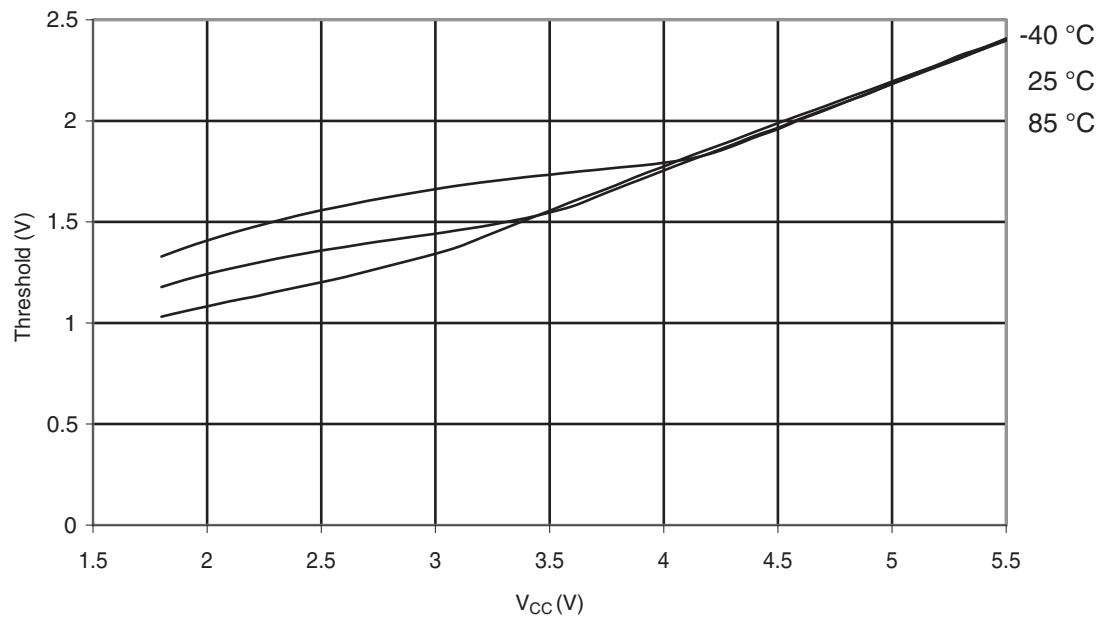
Figure 30-312. ATmega328: Reset Input Threshold Voltage vs. V_{CC} ( V_{IH} , I/O Pin read as '1')
