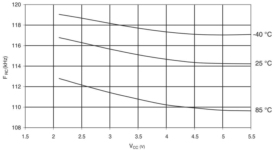
Figure 30-320. ATmega328: Watchdog Oscillator Frequency vs. V_{CC}
