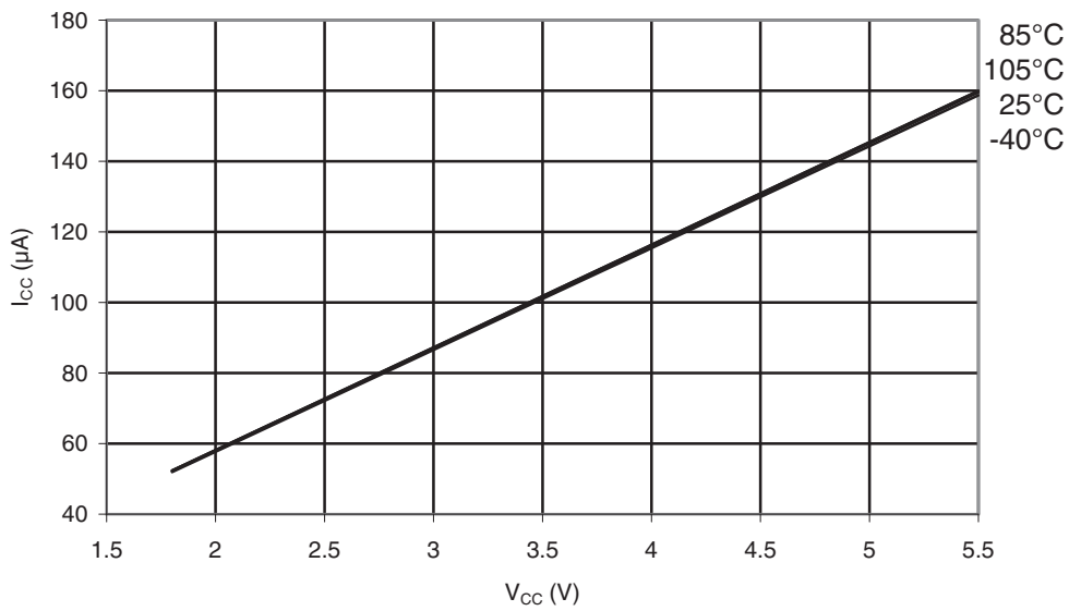
Figure 30-373. ATmega328P: AREF External Reference Current vs. V_{CC}
