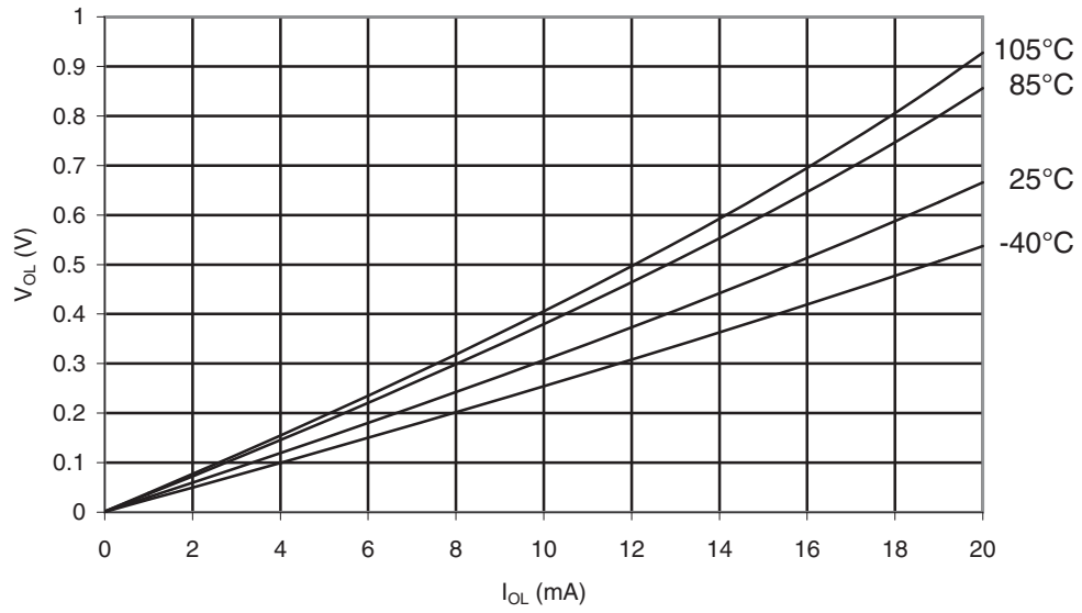
Figure 30-258. ATmega168PA: I/O Pin Output Voltage vs. Sink Current ( V_{CC} = 5V )
