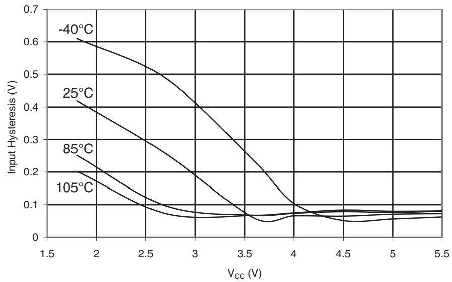
Figure 30-266. ATmega168PA: Reset Pin Input Hysteresis vs. V_{CC}
