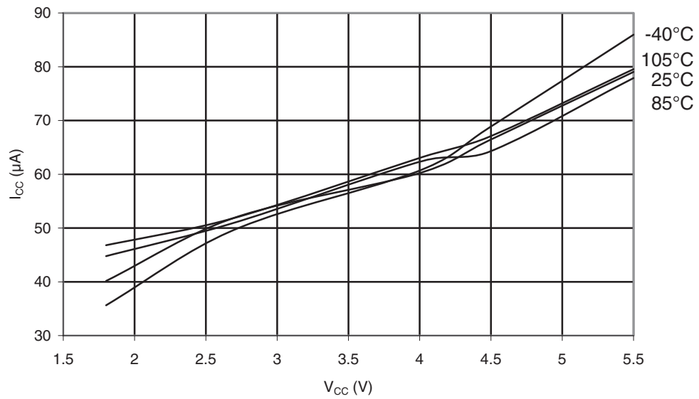
Figure 30-278. ATmega168PA: Analog Comparator Current vs. V_{CC}
