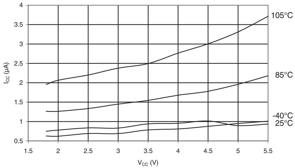
Figure 30-249. ATmega168PA: Power-Save Supply Current vs. V_{CC} (Watchdog Timer Disabled and 32kHz Crystal Oscillator Running)
