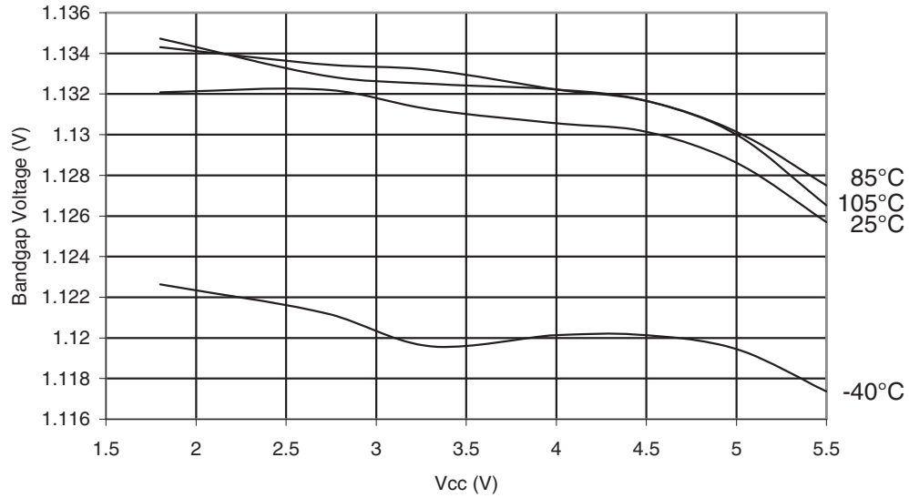
Figure 30-271. ATmega168PA: Calibrated Bandgap Voltage vs. Vcc
