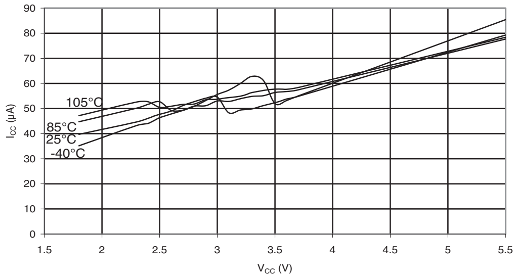
Figure 30-183. ATmega88PA: Analog Comparator Current vs. V_{CC}
