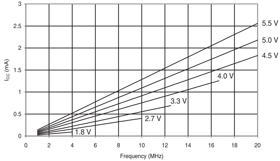
Figure 30-196. ATmega168A: Idle Supply Current vs. Frequency (1-20MHz)
