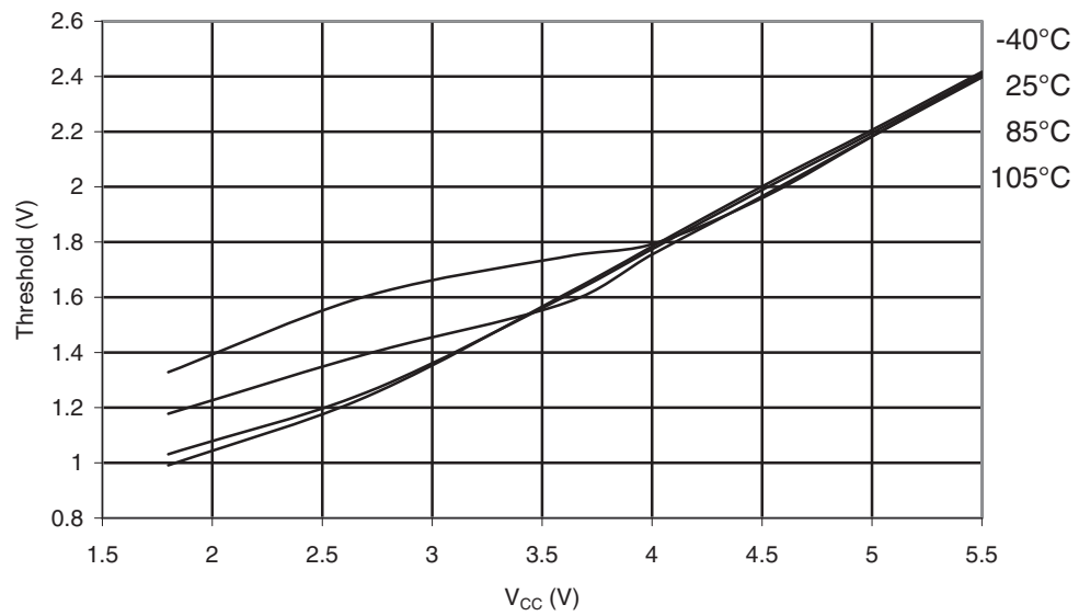
Figure 30-359. ATmega328P: Reset Input Threshold Voltage vs. V_{CC} ( V_{IH} , I/O Pin read as '1')
