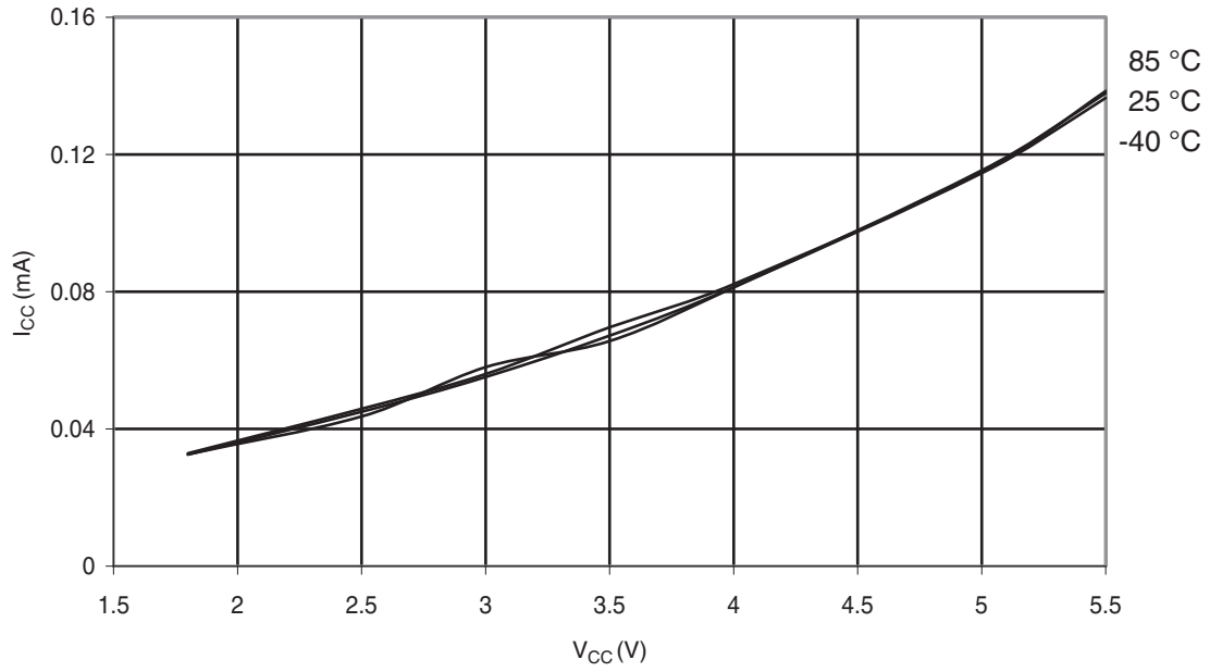
Figure 30-287. ATmega328: Active Supply Current vs. V_{CC} (Internal RC Oscillator, 128kHz)
