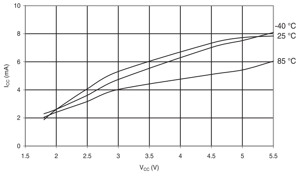
Figure 30-233. ATmega168A: Programming Current vs. V_{CC}
