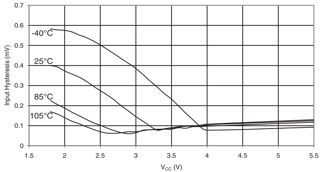
Figure 30-171. ATmega88PA: Reset Pin Input Hysteresis vs. V_{CC}
