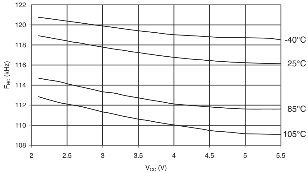
Figure 30-273. ATmega168PA: Watchdog Oscillator Frequency vs. V_{CC}
