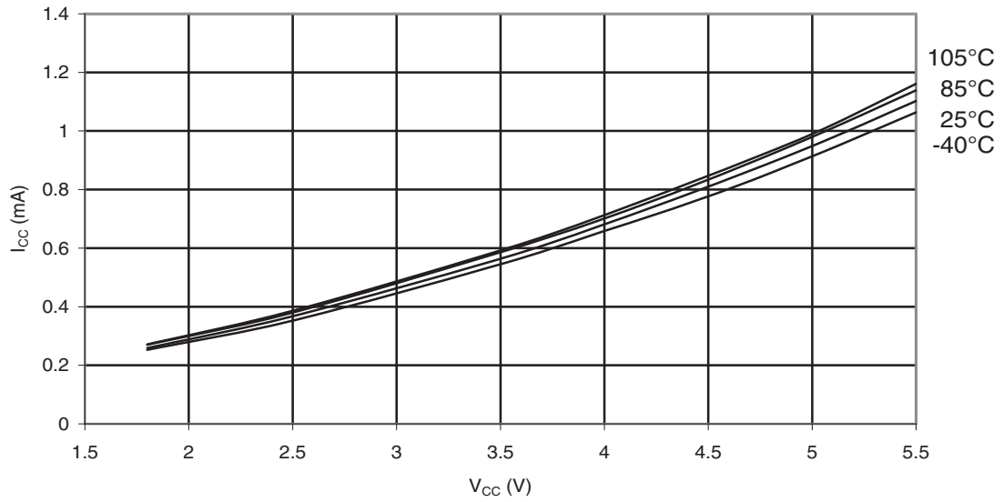
Figure 30-145. ATmega88PA: Active Supply Current vs. V_{CC} (Internal RC Oscillator, 1MHz)
