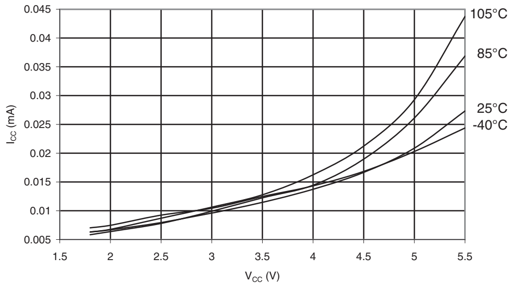
Figure 30-244. ATmega168PA: Idle Supply Current vs. V_{CC} (Internal RC Oscillator, 128kHz)
