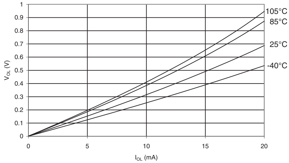
Figure 30-352. ATmega328P: I/O Pin Output Voltage vs. Sink Current ( V_{CC} = 3V )
