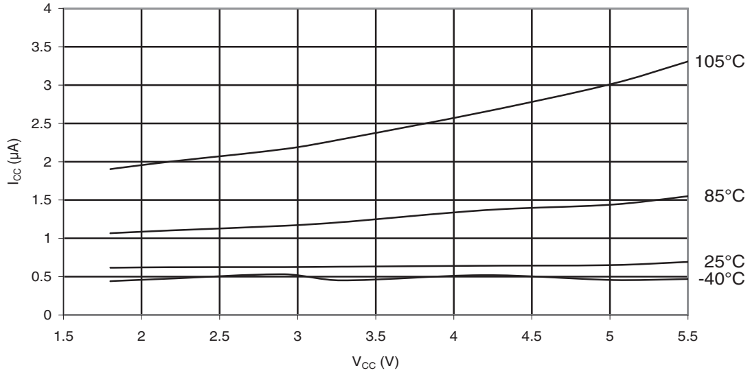
Figure 30-344. ATmega328P: Power-Save Supply Current vs. V_{CC} (Watchdog Timer Disabled and 32kHz Crystal Oscillator Running)
