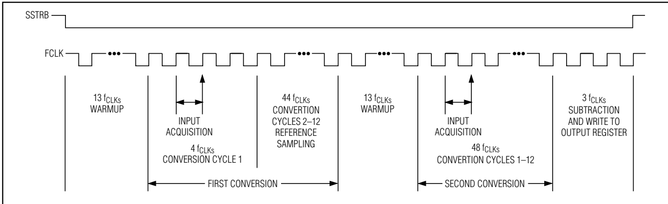
Figure 3b. Temperature Conversion Timing Diagram
