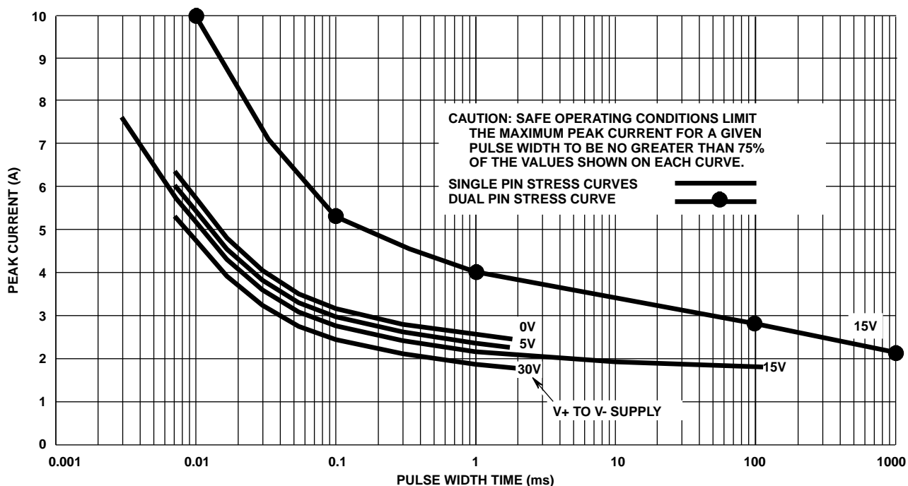
FIGURE 6. SP720 TYPICAL SINGLE PULSE PEAK CURRENT CURVES SHOWING THE MEASURED POINT OF OVER-STRESS IN AMPERES vs PULSE TIME IN MILLISECONDS, (T A = 25°C)
